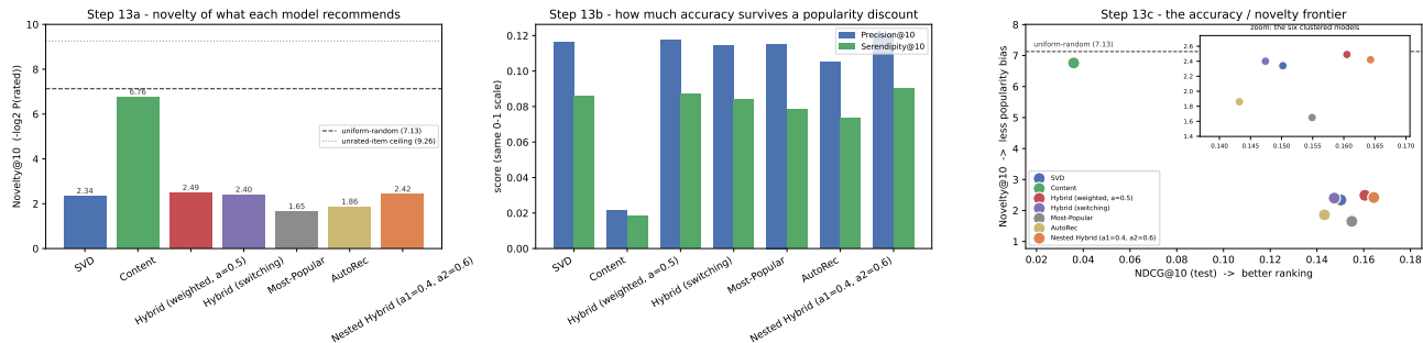
Figure 2. Beyond-accuracy results. Left: novelty of what each model recommends, against the uniform-random line (7.13) and the unrated-item ceiling (9.26). Centre: serendipity beside precision on the same scale. Right: the accuracy/novelty frontier — if any model dominated it would sit alone in the upper right, and none does. The inset zooms the six systems that cluster below the random line.
