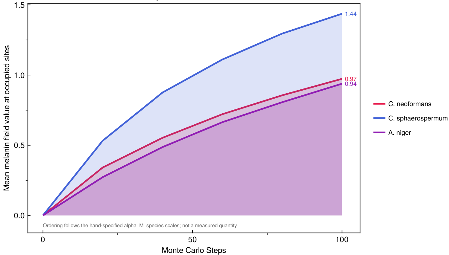
Melanin field at occupied sites — dimensionless model units
