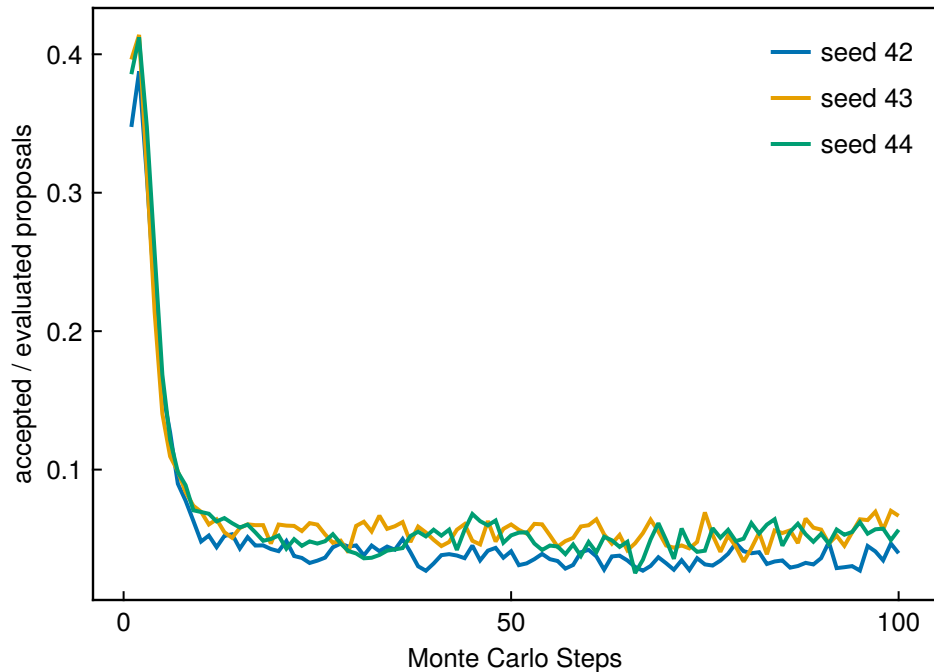
Metropolis acceptance rate per sweep
