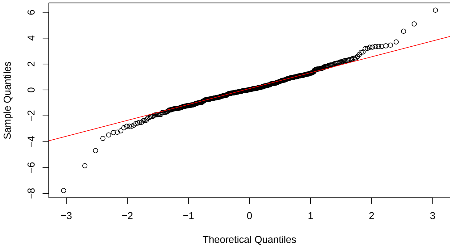
Q-Q Plot of Residuals from Linear Regression
