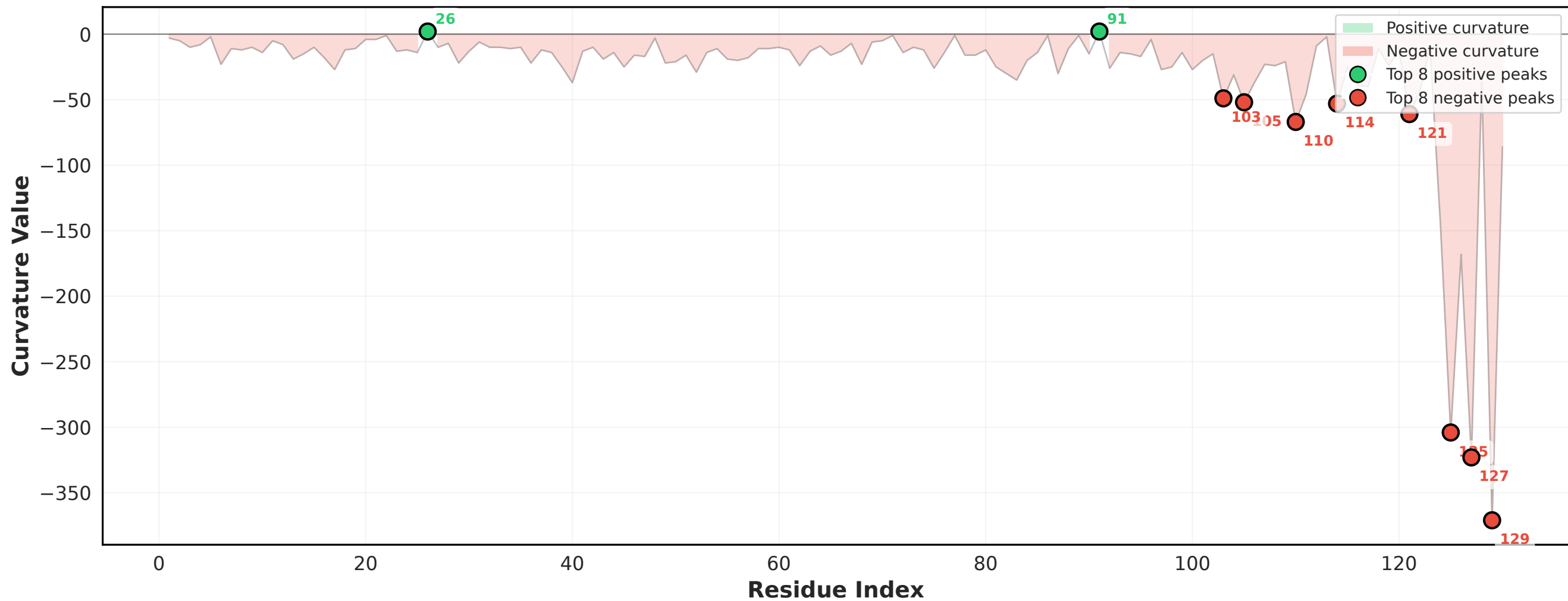
6UEV_A - Curvature Peaks (Top 8 Positive/Negative)
