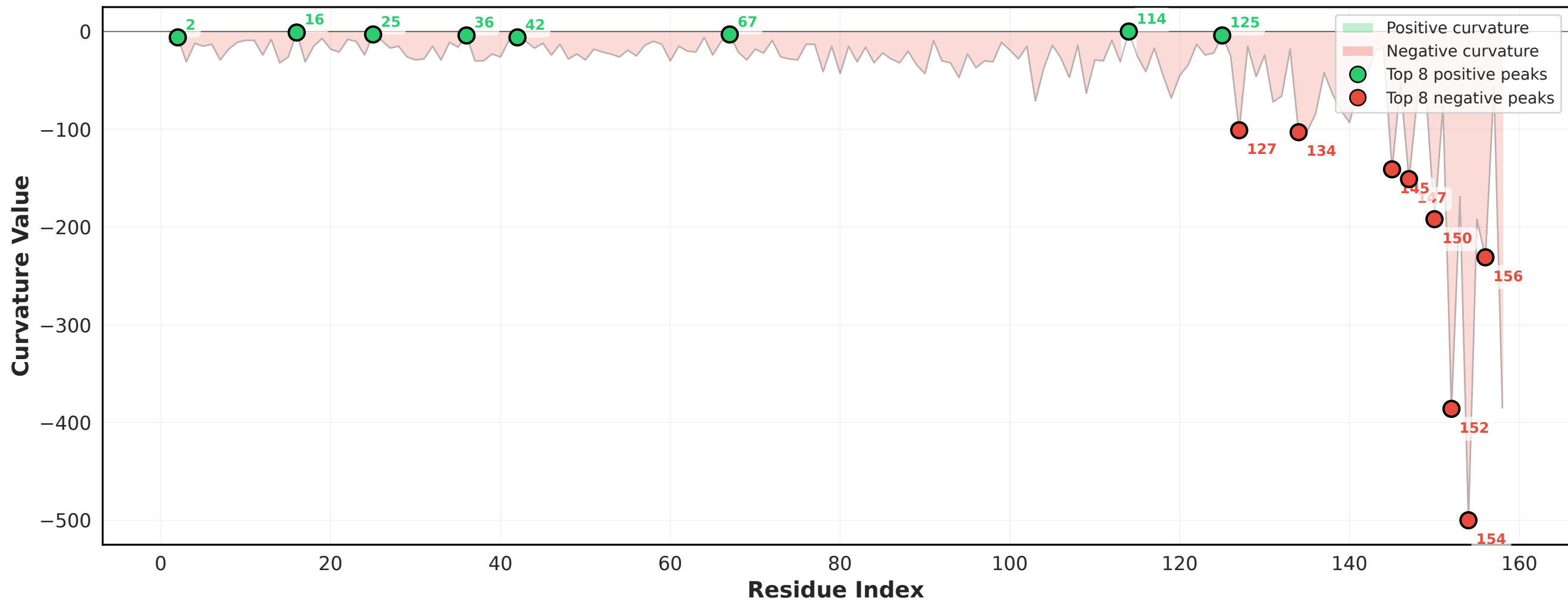
7NH8_A - Curvature Peaks (Top 8 Positive/Negative)
