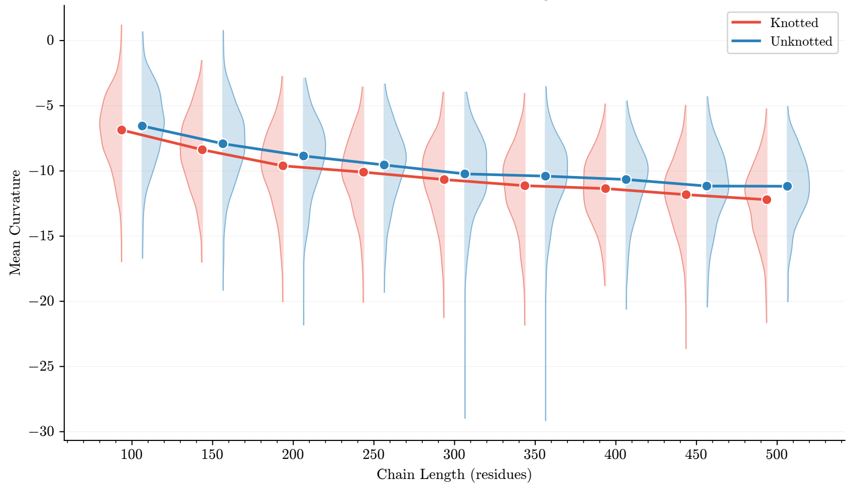
Mean Curvature vs Chain Length
