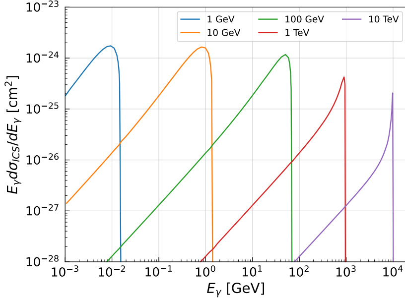
Fig. 2.2. The differential cross section for ICS of a high-energy electron with a 1 eV target photon, for several values of E_e . At high energies ( E_e \gg m_e^2/c^2 ), the process enters the Klein-Nishina regime: the cross section is severely suppressed and the scattered photon carries nearly all the electron's energy.
