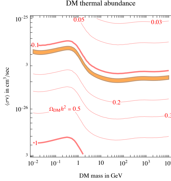
Fig. 1.7. Contours for the dark matter freeze-out abundance \Omega_{\text{DM}} h^2 as a function of DM mass and annihilation cross-section \langle \sigma v \rangle for Majorana dark matter. The measured cosmological abundance \Omega_{\text{DM}} h^2 = 0.120 \pm 0.001 is reproduced within the orange band at 3\sigma . From this plot it is possible to appreciate how the annihilation cross-section needed to match the observed abundance varies with mass in the 1 - 3 \times 10^{-26} \text{ cm}^3/\text{s} range. Credit: Cirelli et al. [11].
