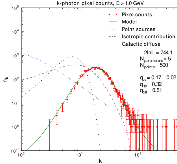
Fig. 6.1. Output of a 1pPDF analysis: photon-count statistics of the high-latitude Fermi-LAT sky above 1 GeV. The red points show the measured n_k , the number of pixels containing exactly k photons, together with the best-fit model (solid green) and its decomposition into point sources (dotted blue), Galactic diffuse emission (dashed brown), and the isotropic background (dot-dashed black). Credit: Malyshev and Hogg [322].
