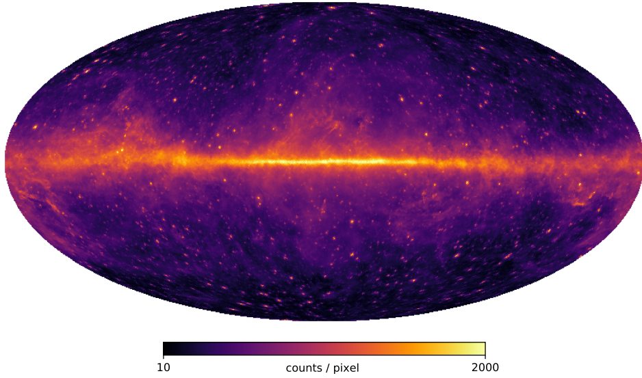
Fig. 6.9. Simulated count map in units of counts per pixel, at the Healpix resolution N_{\text{side}} = 128 ( n = 7 ).
