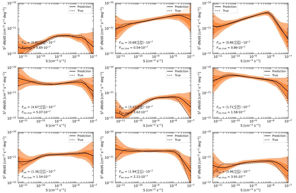
Fig. 6.28. Some example dN/dS from the validation dataset of the spherical CNN. Each panel shows the input dN/dS and F_{\text{iso}} and the corresponding quantities reconstructed by the CNN. The colored areas indicate the 1\sigma and 2\sigma uncertainty bands.
