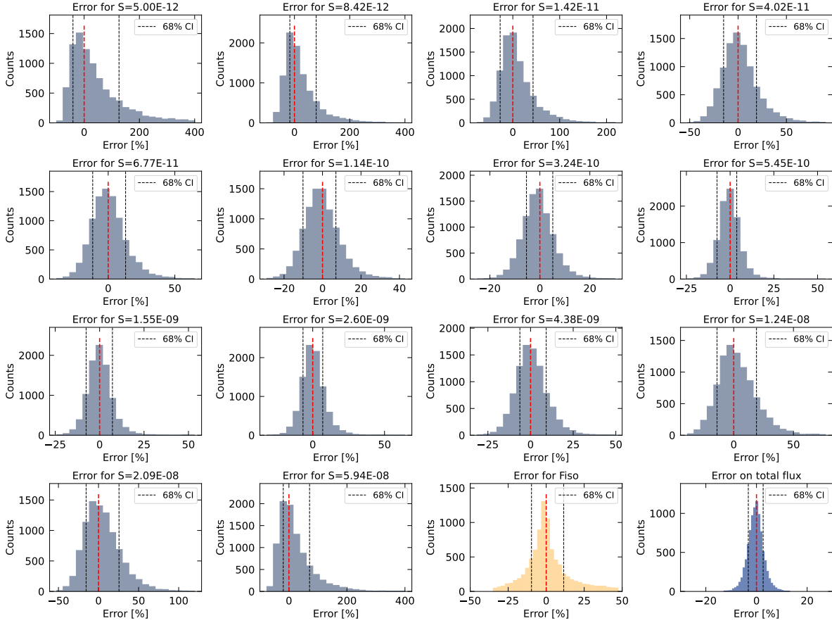
Fig. 6.13. Histograms of the percentage deviations between the true and reconstructed dN/dS for 14 values of S across its interval of interest, and for F_{\text{iso}} . The bottom right panel shows the same, but for a derived quantity, namely the total flux. The dotted vertical black lines indicate the 68% confidence region.
