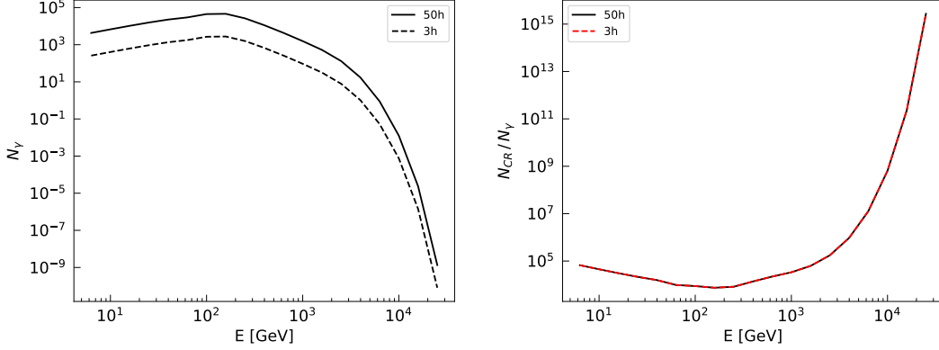
Fig. 8.12. Left: Number of expected \gamma -ray events N_\gamma in the CTAO survey as a function of energy. Right: Ratio of cosmic-ray events to expected \gamma -ray events ( N_{\text{CR}}/N_\gamma ) after quality cuts in the CTAO survey. The ratio worsens above 1 TeV due to significant \gamma -ray suppression from EBL attenuation. N_\gamma is determined for the HSP plus LISP source classes.
