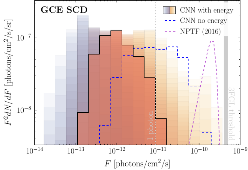
Fig. 4.2. SCD of the GCE inferred via three approaches. The NPTF (dashed purple) placed the emission just below the Fermi 3FGL detection threshold; an energy-independent CNN (dashed blue) preferred a somewhat fainter population. Including energy information (solid black, with quantile bands from purple to orange) drives the SCD below the one-photon line. At this level, at 95% confidence, only 3% of the emission can be excluded as Poissonian. From [231], Figure 1 (right panel).
