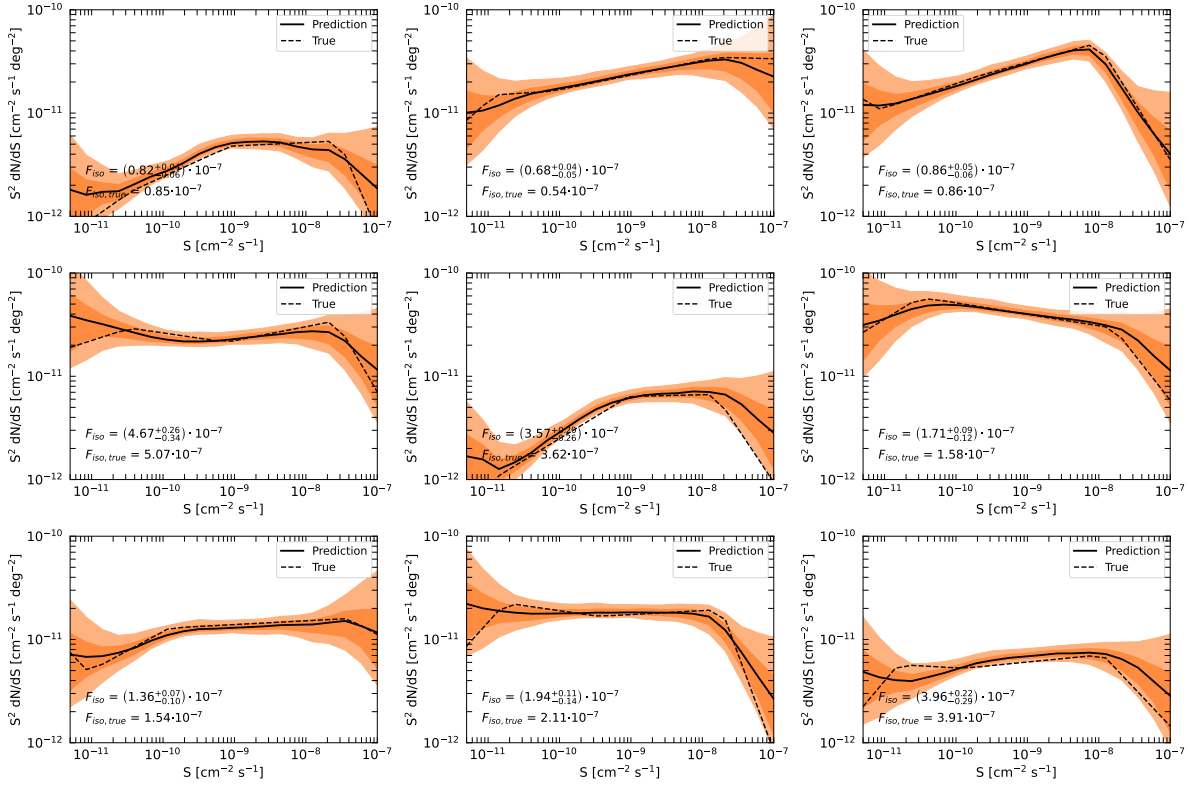
Fig. 6.28. Some example dN/dS from the validation dataset of the spherical CNN. Each panel shows the input dN/dS and F_{\text{iso}} and the corresponding quantities reconstructed by the CNN. The colored areas indicate the 1 \sigma and 2 \sigma uncertainty bands.
