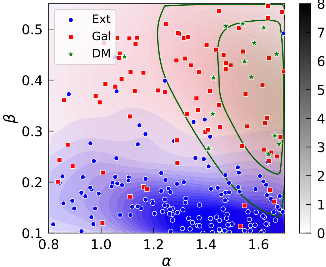
True classes
