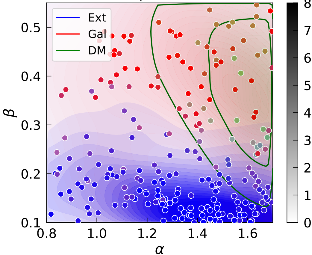
Class probabilities
