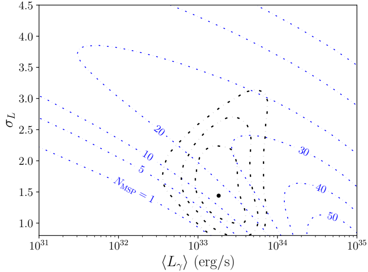
Fig. 4.7. As in Figure 4.6, but for the best fit model including cluster-to-cluster variations. The results are compatible with the estimates in Figure 4.6 within the 1\sigma band, although the model with cluster-to-cluster variations favors lower values for \langle L_\gamma \rangle and \sigma_L .
