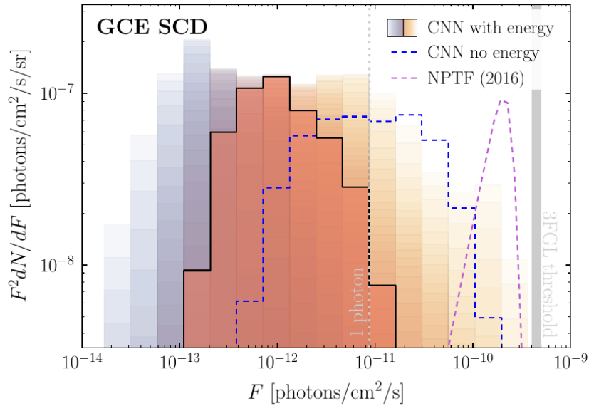
Fig. 4.1. Source-count distribution (SCD) of the GCE inferred via three approaches. The NPTF (dashed purple) placed the emission just below the Fermi 3FGL detection threshold; an energy-independent CNN (dashed blue) preferred a somewhat fainter population. Including energy information (solid black, with quantile bands from purple to orange) drives the SCD below the one-photon line. At this level, at 95% confidence, only 3% of the emission can be excluded as Poissonian. From [94], Figure 1 (right panel).
