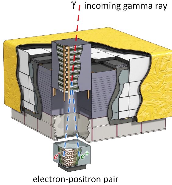
Fig. 2.5. Schematic diagram of the Large Area Telescope, showing the tracker modules, calorimeter, and the surrounding Anticoincidence Detector. The telescope’s dimensions are 1.8 \text{ m} \times 1.8 \text{ m} \times 0.72 \text{ m} . Adapted from Figure 1 from [16].
