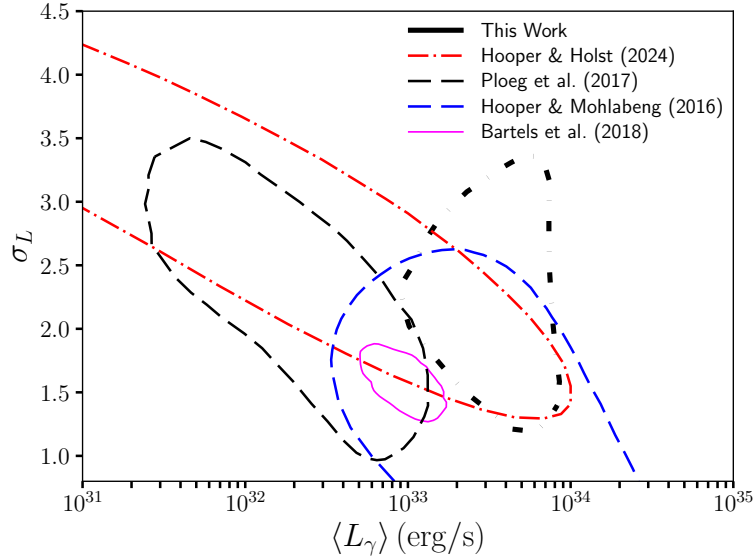
Fig. 4.5. A comparison of the 2\sigma constraints on the MSP gamma-ray luminosity found in this study (for the best-fitting case of \langle N_{\text{MSP}} \rangle = R_{\text{MSP}} \Gamma_e^{0.7} + R'_{\text{MSP}} L_V ) to those published in previous studies of MSPs in the Galactic Plane. The luminosity function preferred by our analysis is in good agreement with those derived by Holst and Hooper [77], and by Hooper and Mohlabeng [76], but favor somewhat larger values for the average MSP luminosity than Ploeg et al. [116], or Bartels et al. [117].
