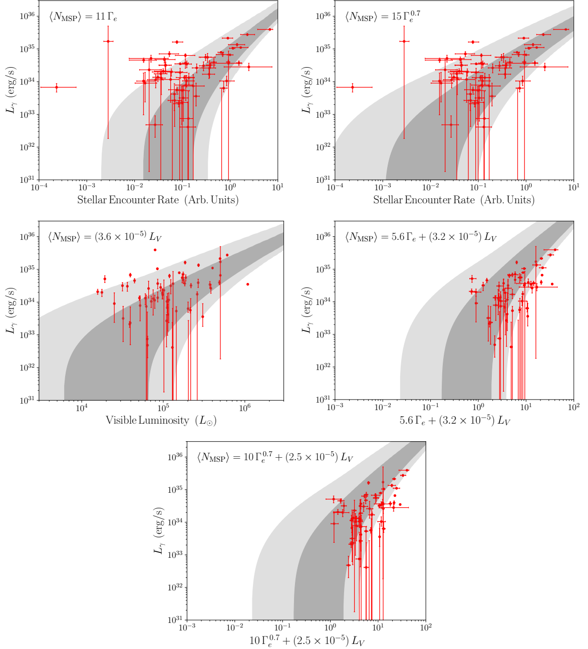
Fig. 4.3. The measured gamma-ray luminosities of the 87 globular clusters considered in this study (those with L_V > 10^5 L_\odot or \Gamma_e > 0.01 ), compared to combinations of their stellar encounter rates and/or visible luminosities. As dark (light) grey bands, we show the 68.27% (95.45%) confidence interval predicted by the model for the total gamma-ray luminosity. In each frame, we show the results that were obtained using the best-fit values for \langle L_\gamma \rangle , \sigma_L , R_{\text{MSP}} , and/or R'_{\text{MSP}} (see Table 4.2).
