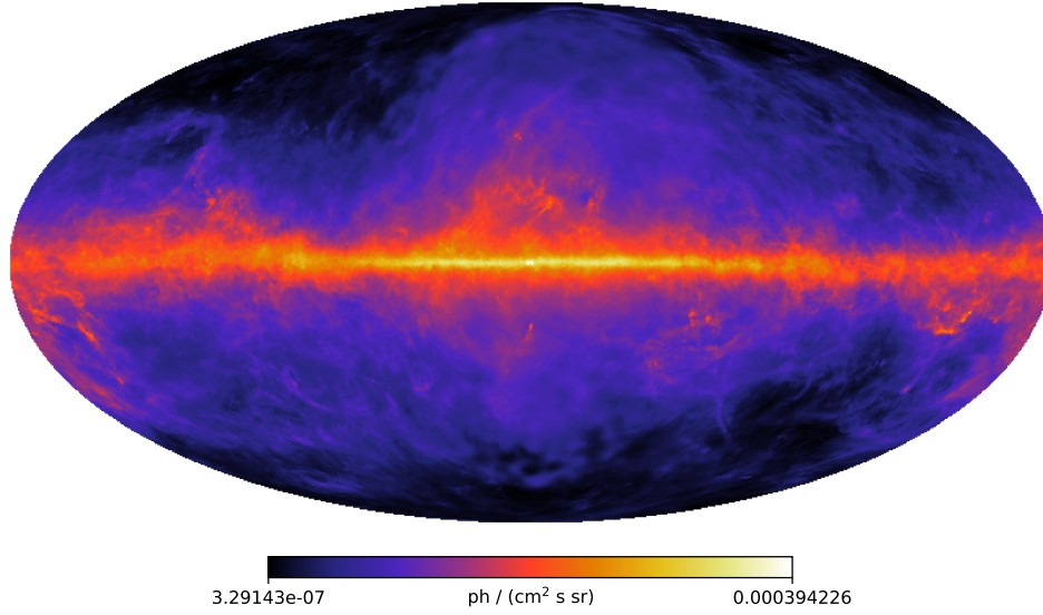
Fig. 6.6. gll_iem_v07 galactic foreground model [20], integrated in the (1, 10) GeV energy bin, in units of photons/(cm 2 s sr), at the Healpix resolution N_{\text{side}} = 128 ( n = 7 ).
