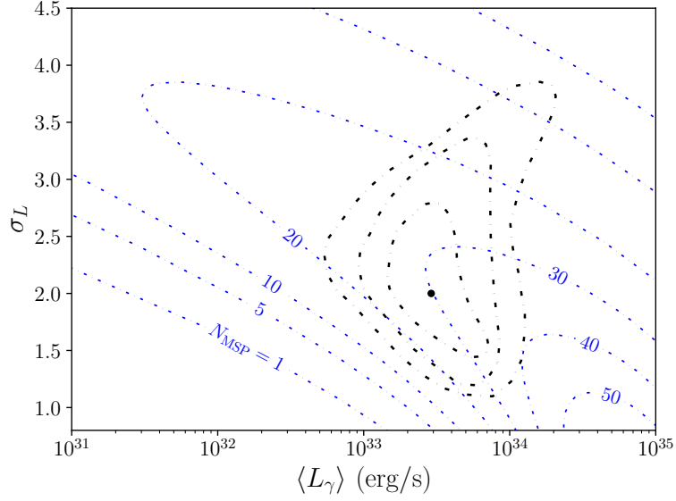
Fig. 4.6. The constraints on the MSP gamma-ray luminosity found in this study (shown for the case of \langle N_{\text{MSP}} \rangle = R_{\text{MSP}} \Gamma_e^{0.7} + R'_{\text{MSP}} L_V ), shown along with contours representing the number of Inner Galaxy MSPs that should appear in the Fermi source catalogs, N_{\text{MSP}} , assuming that the Galactic Center Gamma-Ray Excess (GCE) is generated by MSPs [77]. As there are only three Inner Galaxy pulsars candidates in the 3PC, MSPs can generate the excess gamma-ray emission only if that source population consists of members that are significantly less luminous than those present in globular clusters.
