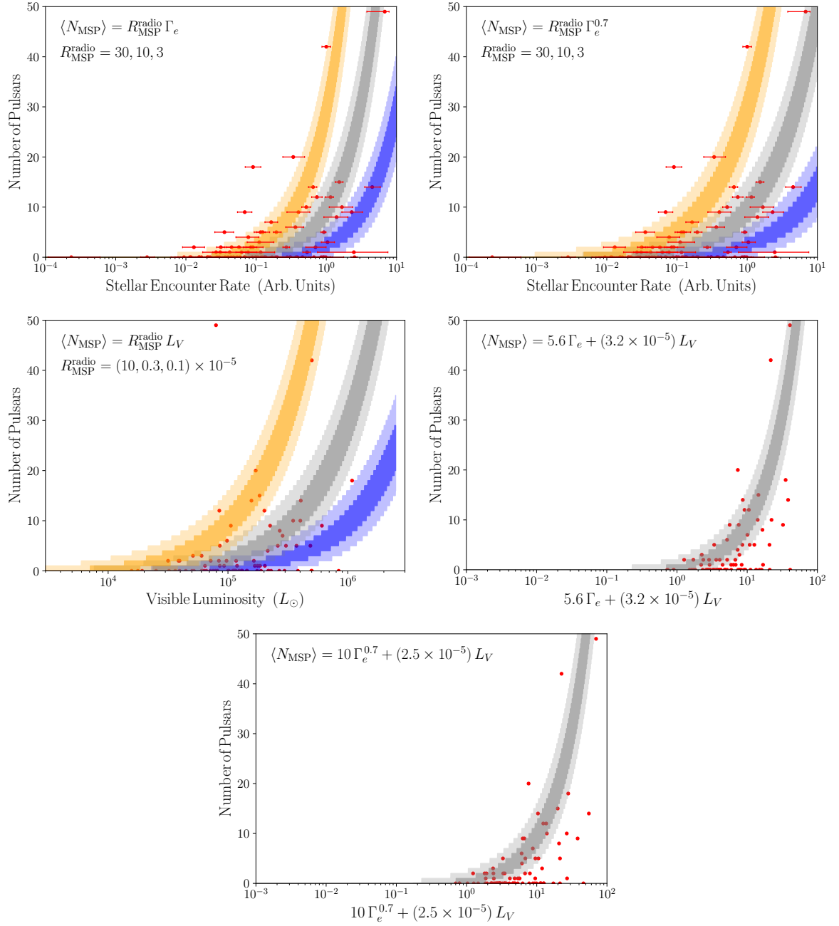
Fig. 4.2. The number of known millisecond pulsars in each of the 87 globular clusters considered in this study (those with L_V > 10^5 L_\odot or \Gamma_e > 0.01 ) as a function of combinations of the stellar encounter rate, \Gamma_e , and visible luminosity, L_V (in units of solar luminosities). Also shown are colored bands representing the predicted number of MSPs (68.27% and 95.45% containment) in each case, for selected values of R_{\text{MSP}}^{\text{Radio}} . The stellar encounter rate is normalized such that \Gamma_e = 1 for NGC 104.
