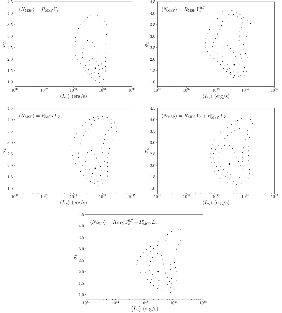
Fig. 4.4. Constraints on the MSP gamma-ray luminosity function parameters, after marginalizing over R_{\text{MSP}} and/or R'_{\text{MSP}} . The best-fit point in each frame is shown as a dot, while the contours reflect the regions that are preferred at the levels of 1, 2 and 3 \sigma confidence.
