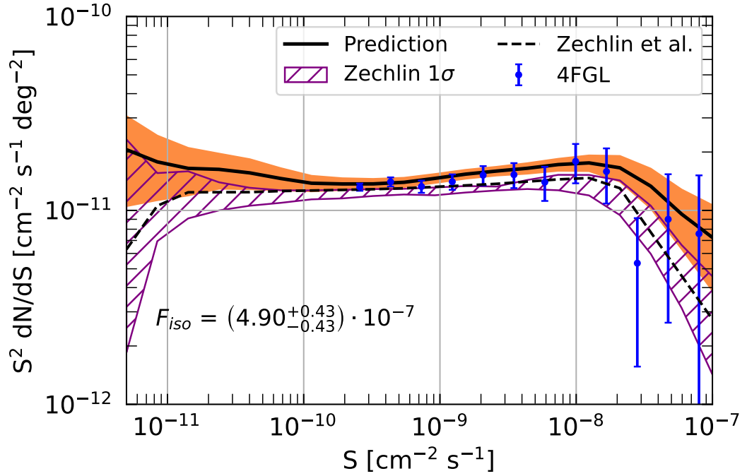
Fig. 6.15. Same as Figure 6.14, including a comparison with the result of Ref. [183].
