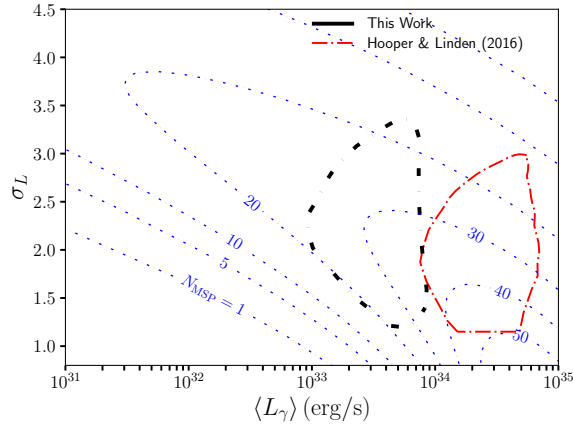
Fig. 4.8. As in Figure 4.6, for the 2\sigma contours, but comparing the results from the prior 2016 work from Hooper and Linden [76] with our most recent findings.
