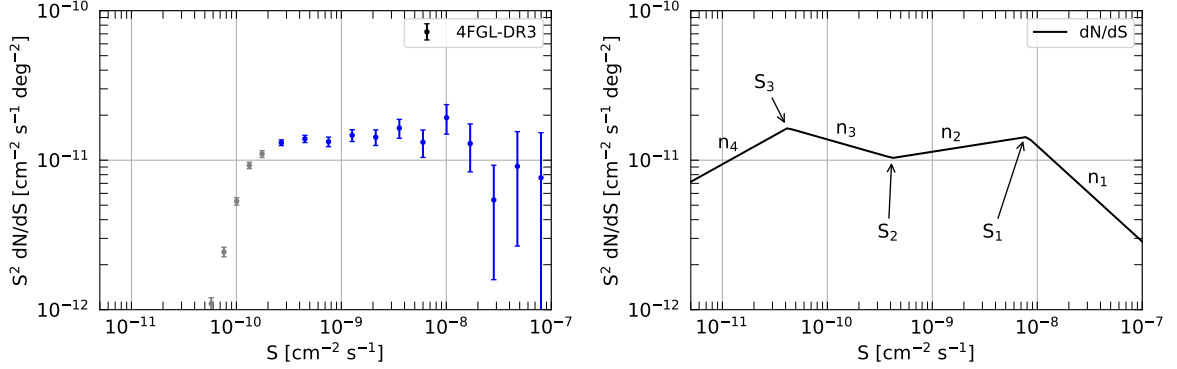
Fig. 6.4. Left: The 1-10 GeV \text{dN/dS} for resolved Fermi -LAT sources, obtained from the 4FGL-DR3 [133] catalog. Right: An example of \text{dN/dS} with 3 breaks S_j ( j = 1, 3 ) and four slopes, where n_i ( i = 1, 4 ) is the inclination of the slope.
