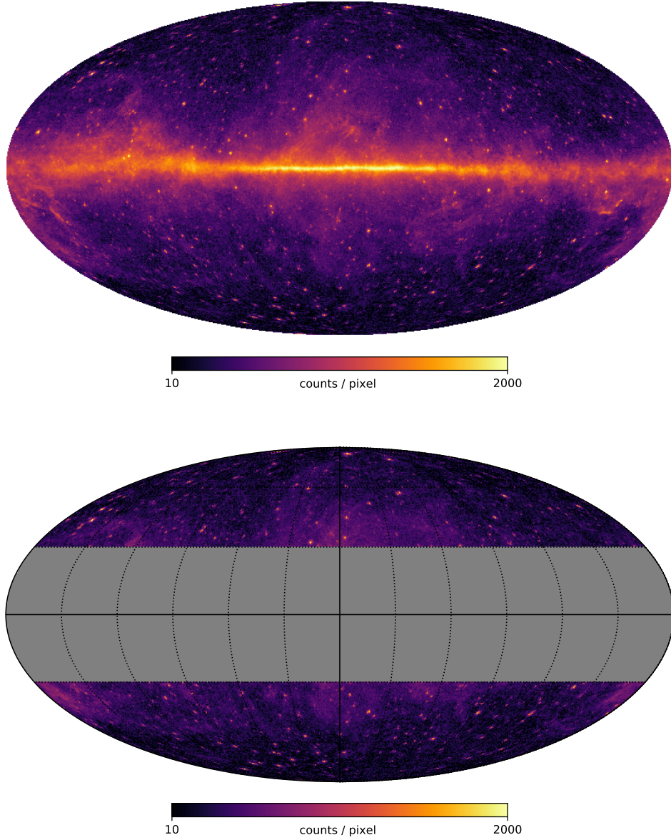
Fig. 6.9. Simulated map in units of counts per pixel after adding Poisson noise from the synthetic model map of Figure 6.8, at the same Healpix resolution N_{\text{side}} = 128 ( n = 7 ). The lower panel shows the map with a |b| < 30^\circ latitude cut.
