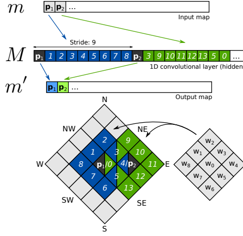
(b) Unrolled convolution scheme.
