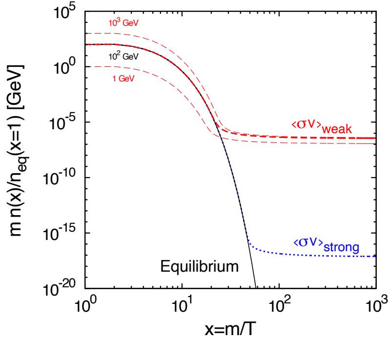
Fig. 1.6. Freeze-out of a thermal relic as a function of the dimensionless inverse temperature x \equiv M_\chi/T . The vertical axis is M_\chi n(x)/n_{\text{eq}}(x=1) (in GeV), i.e. the mass times the comoving number density normalised to the equilibrium value at x = 1 . Up to a constant this is proportional to M_\chi Y , with Y \equiv n_\chi/s the comoving abundance, so that the post-freeze-out plateau measures the relic mass density directly and hence \Omega_\chi h^2 . The solid black curve traces the equilibrium abundance, exponentially Boltzmann-suppressed once T falls below M_\chi ( x \gtrsim 1 ): while annihilations remain faster than the Hubble rate the abundance tracks equilibrium, and once they become inefficient it freezes out at a constant comoving value. The thick red (dashed) curve corresponds to a weak-scale cross section \langle\sigma v\rangle_{\text{weak}} , shown as a band for WIMP masses of 1, 10^2 and 10^3 GeV to illustrate the near mass-independence of the freeze-out, while the blue (dotted) curve shows a much larger \langle\sigma v\rangle_{\text{strong}} : a stronger annihilation cross section tracks equilibrium longer and freezes out at a smaller residual abundance ( Y_\infty \propto 1/\langle\sigma v\rangle ). Credit: Steigman et al. [12].
