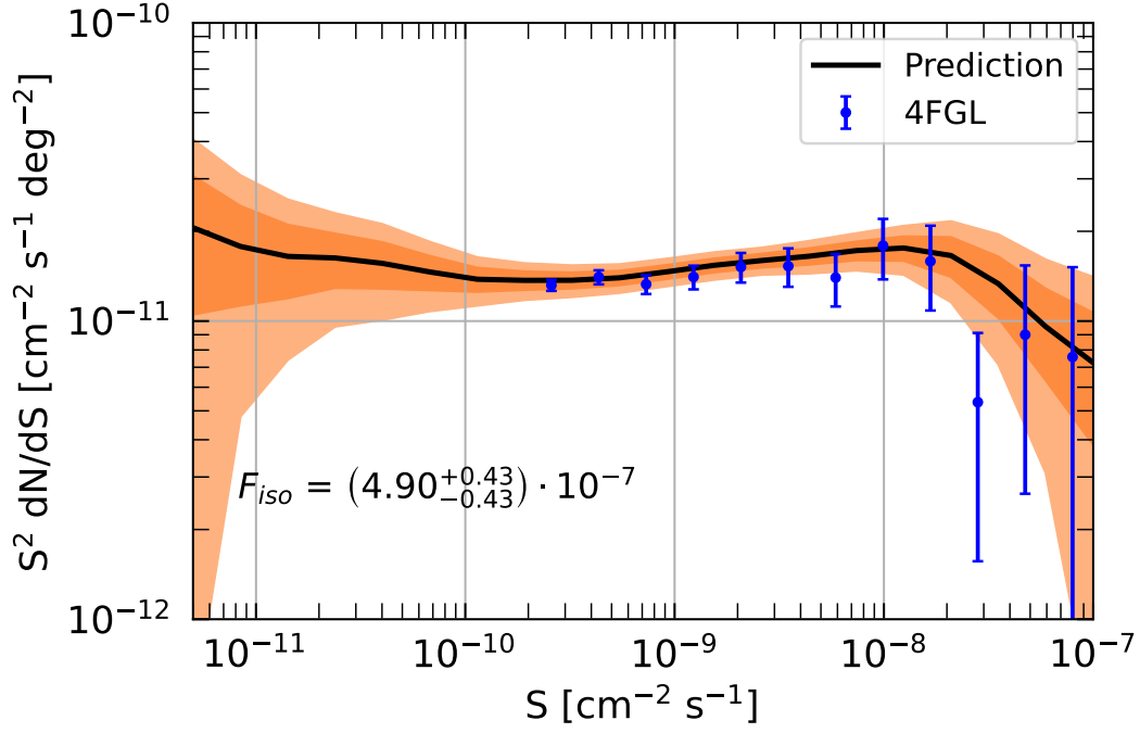
Fig. 6.15. Reconstructed dN/dS and F_{iso} and their Bayesian errors, when the trained CNN is applied to the Fermi -LAT map. This is the main baseline result of the analysis.
