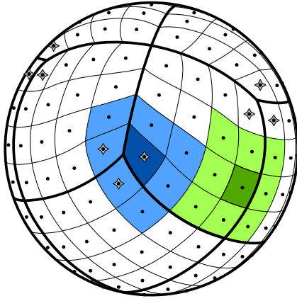
(a) Pixel neighbourhood on the HEALPix sphere.
