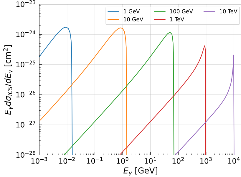
Fig. 2.2. The differential cross section for inverse Compton scattering of a high-energy electron with a 1 eV target photon, for several values of E_e . At high energies ( E_e \gg m_e^2/c^2 ), the process enters the Klein-Nishina regime: the cross section is severely suppressed and the scattered photon carries nearly all the electron’s energy.
