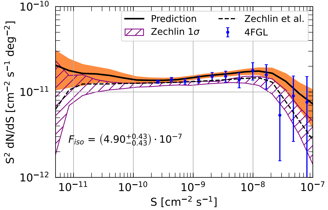
Fig. 6.16. Same as Figure 6.15, including a comparison with the result of Ref. [308].
