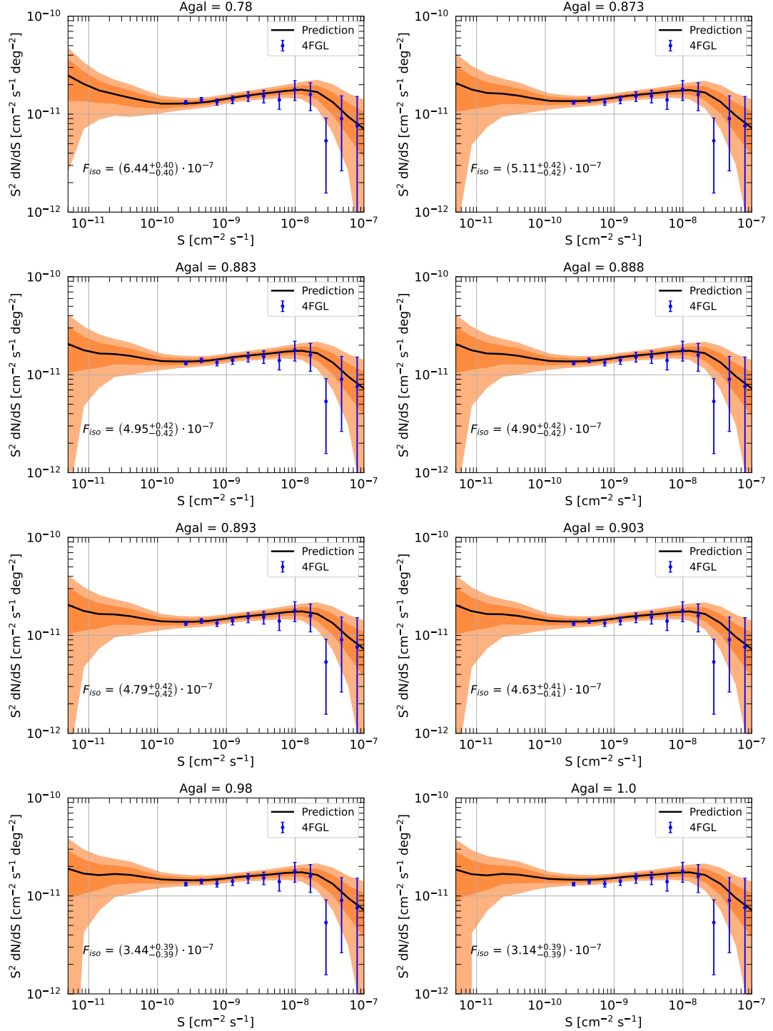
Fig. 6.26. Reconstructed dN/dS and F_{iso} and their Bayesian errors, when the trained CNN is applied to the Fermi -LAT map using different values of A_{gal} as indicated in the panel labels.
