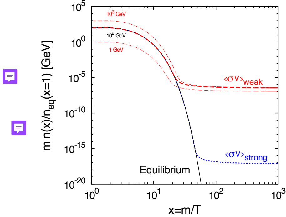
Fig. 1.6. Freeze-out of a thermal relic as a function of the dimensionless inverse temperature x \equiv M_\chi/T . The vertical axis is M_\chi n(x)/n_{\text{eq}}(x=1) (in GeV), i.e. the mass times the comoving number density normalised to the equilibrium value at x = 1 . Up to a constant this is proportional to M_\chi Y , with Y \equiv n_\chi/s the comoving abundance, so that the post-freeze-out plateau measures the relic mass density directly and hence \Omega_\chi h^2 . The solid black curve traces the equilibrium abundance, exponentially Boltzmann-suppressed once T falls below M_\chi ( x \gtrsim 1 ): while annihilations remain faster than the Hubble rate the abundance tracks equilibrium, and once they become inefficient it freezes out at a constant comoving value. The thick red (dashed) curve corresponds to a weak-scale cross section \langle\sigma v\rangle_{\text{weak}} , shown as a band for WIMP masses of 1, 10^2 and 10^3 GeV to illustrate the near mass-independence of the freeze-out, while the blue (dotted) curve shows a much larger \langle\sigma v\rangle_{\text{strong}} : a stronger annihilation cross section tracks equilibrium longer and freezes out at a smaller residual abundance ( Y_\infty \propto 1/\langle\sigma v\rangle ). Credit: Steigman et al. [12].
