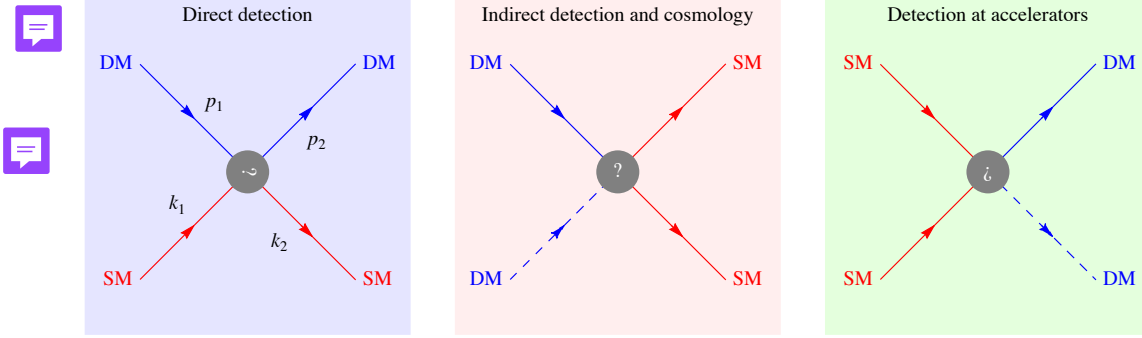
Fig. 1.8. The detection triangle: three complementary strategies for detecting dark matter, each corresponding to a different reading of the same underlying interaction vertex. Left : direct detection — dark matter scatters off a Standard Model target in a laboratory. Center : indirect detection — dark matter annihilates or decays into Standard Model particles in astrophysical environments. In decay, the process involves a single dark matter particle, thus the dashed line. Right : collider production — Standard Model particles produce dark matter at accelerators. A dashed line indicates that the process might involve production of just one dark matter particle. Credit: Cirelli et al. [11].
