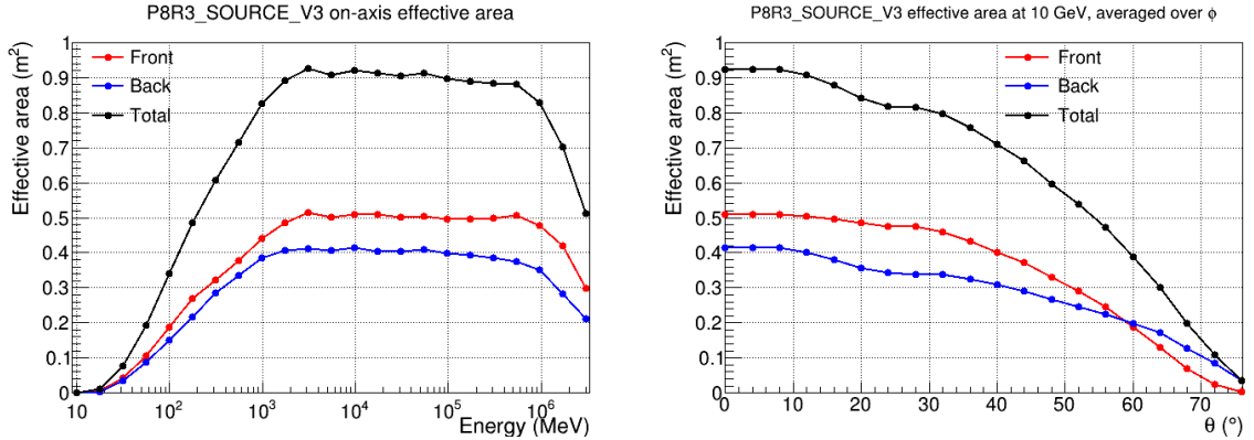
Fig. 2.6. Left: Effective area as a function of the energy of the incident photon. Right: Effective area at 10 GeV as a function of the angle of incidence. Credit: Fermi-LAT collaboration [142].
