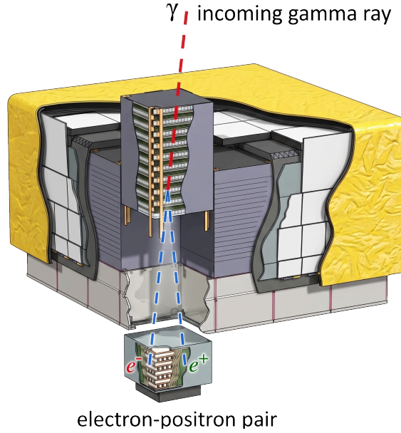
Fig. 2.4. Schematic diagram of the Large Area Telescope, showing the tracker modules, calorimeter, and the surrounding Anticoincidence Detector. The telescope’s dimensions are 1.8 \text{ m} \times 1.8 \text{ m} \times 0.72 \text{ m} . Adapted from Figure 1 from [141].
