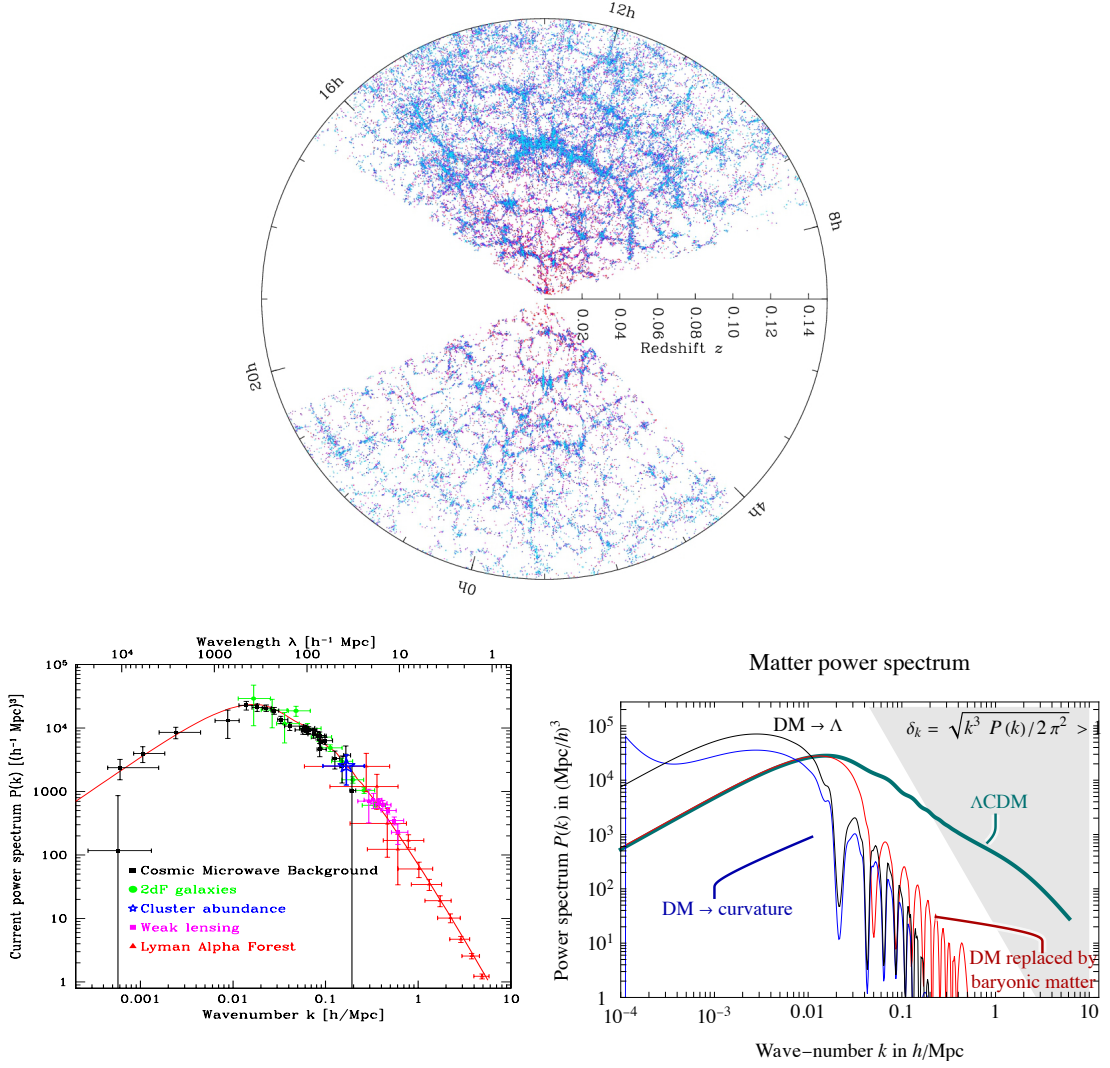
Fig. 1.4. The imprint of dark matter on large-scale structure. Top: the large-scale distribution of galaxies from the Sloan Digital Sky Survey (SDSS) [30]. Bottom left: the observed matter power spectrum P(k) [31]. Bottom right: the same quantity computed in several different cosmological scenarios. The green line represents the best-fit \Lambda CDM model, while the red line shows the prediction for a universe without cold dark matter, in which power on small (large- k ) scales is strongly suppressed — reflecting the absence of small-scale structure [32]. Adapted from the SDSS Collaboration [30], Tegmark and Zaldarriaga [31], and Cirelli et al. [11].
