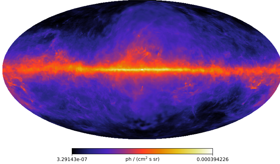
Fig. 6.7. gll_iem_v07 galactic foreground model [134], integrated in the (1, 10) GeV energy bin, in units of photons/(cm 2 s sr), at the Healpix resolution N_{\text{side}} = 128 ( n = 7 ).
