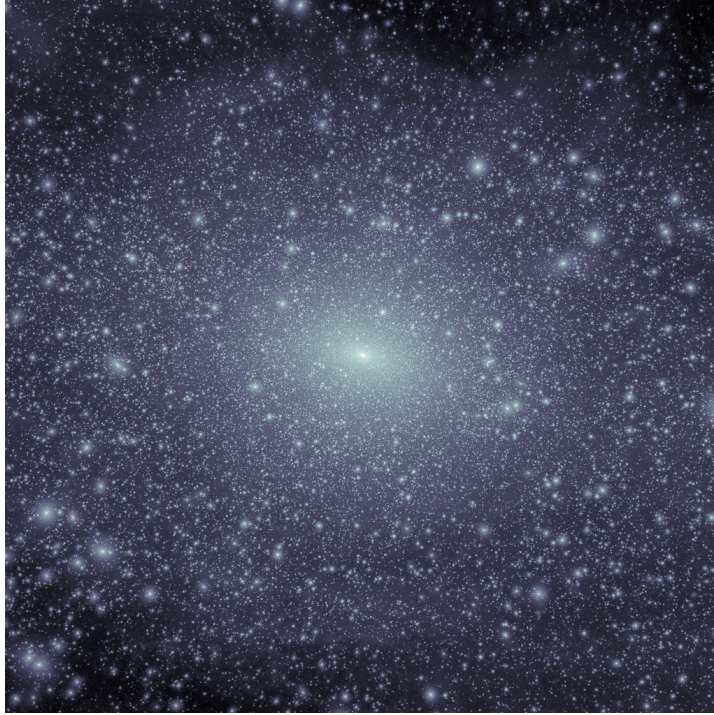
Fig. 5.1. Dark matter substructure in a Milky Way-like halo from the Via Lactea II N -body simulation [109], illustrating the vast population of subhalos predicted by \Lambda CDM. The map shows the local dark matter density at z = 0 within an 800 kpc cube. Credit: Diemand et al. [109].
