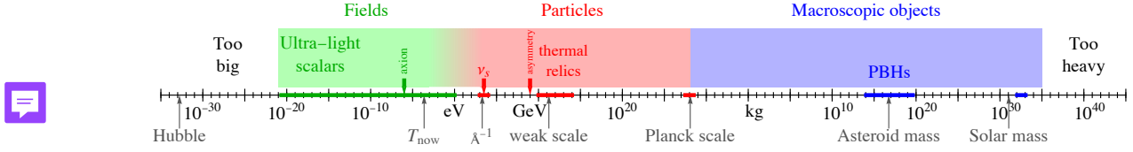
Fig. 1.5. The dark-matter mass landscape: viable candidate masses span roughly ninety orders of magnitude, from ultra-light bosonic fields to macroscopic primordial black holes. Each class is characterized by a distinct production mechanism and probed by a complementary set of experiments. Credit: Cirelli et al. [11]. [AA: consider replacing with a custom figure for the final version]
