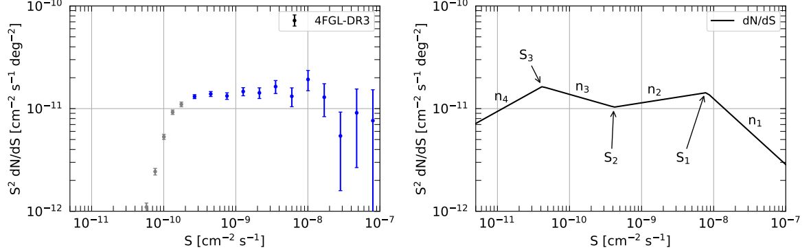
Fig. 6.5. Left: The 1-10 GeV dN/dS for resolved Fermi -LAT sources, obtained from the 4FGL-DR3 [135] catalog. Right: An example of dN/dS with 3 breaks S_j ( j = 1, 3 ) and four slopes, where n_i ( i = 1, 4 ) is the inclination of the slope.
