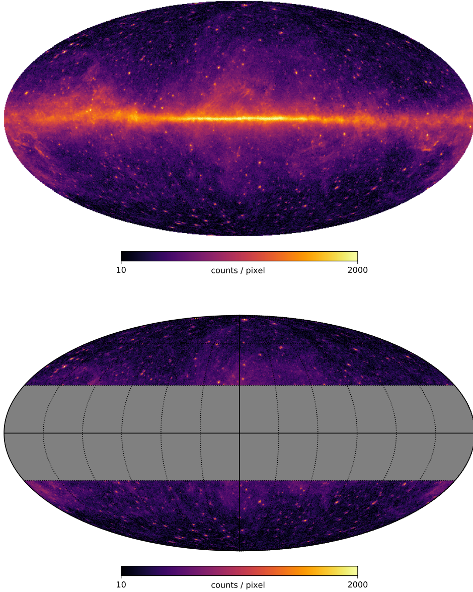
Fig. 6.10. Simulated map in units of counts per pixel after adding Poisson noise from the synthetic model map of Figure 6.9, at the same Healpix resolution N_{\text{side}} = 128 ( n = 7 ). The lower panel shows the map with a |b| < 30^\circ latitude cut.
