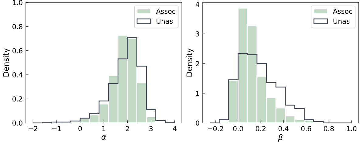
Fig. 3.3. Distributions of the spectral index \alpha and spectral curvature \beta for associated (green, filled) and unassociated (gray outline) Fermi-LAT sources from the 4FGL-DR4 catalog. The visible mismatch between the two populations illustrates the dataset shift between the associated and unassociated samples discussed in Section 3.4.1. The full analysis is presented in Chapter 5.
