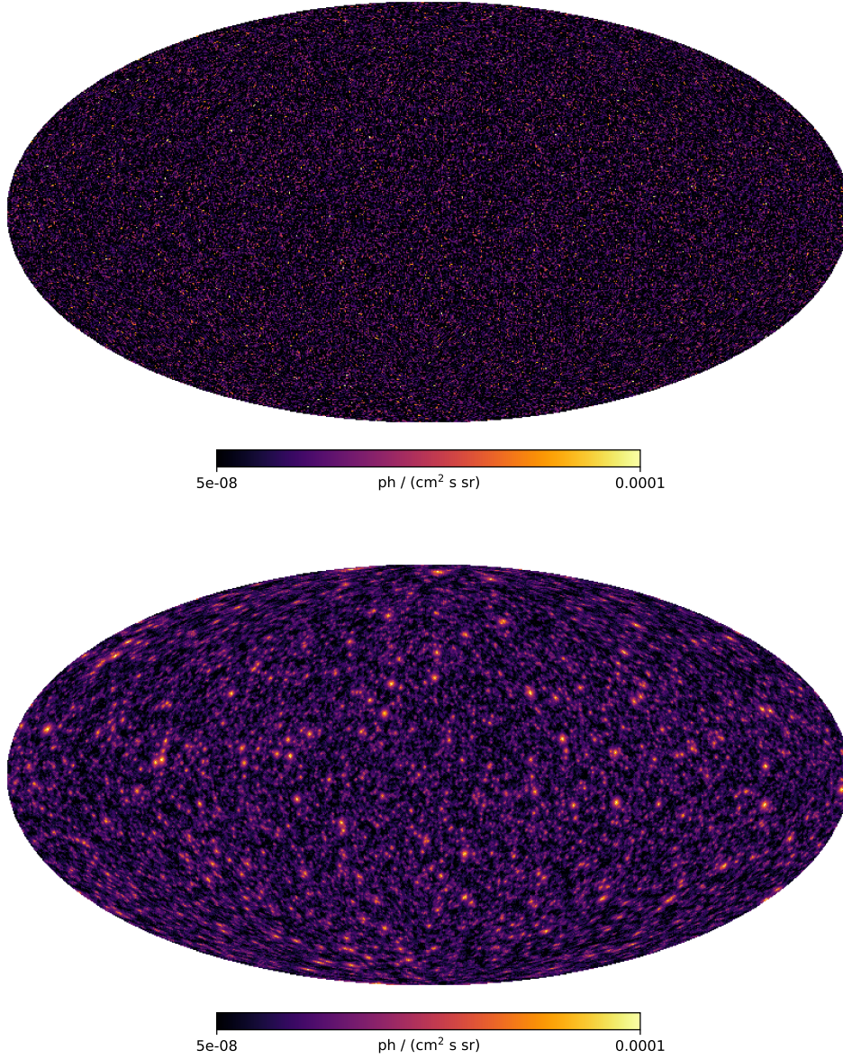
Fig. 6.6. Simulated flux map of point sources extracted from a specific source-count distribution, before (upper panel) and after (lower panel) the PSF is applied, in units of photons/(cm 2 s sr). The maps are shown at Healpix resolution N_{\text{side}} = 128 ( n = 7 ).
