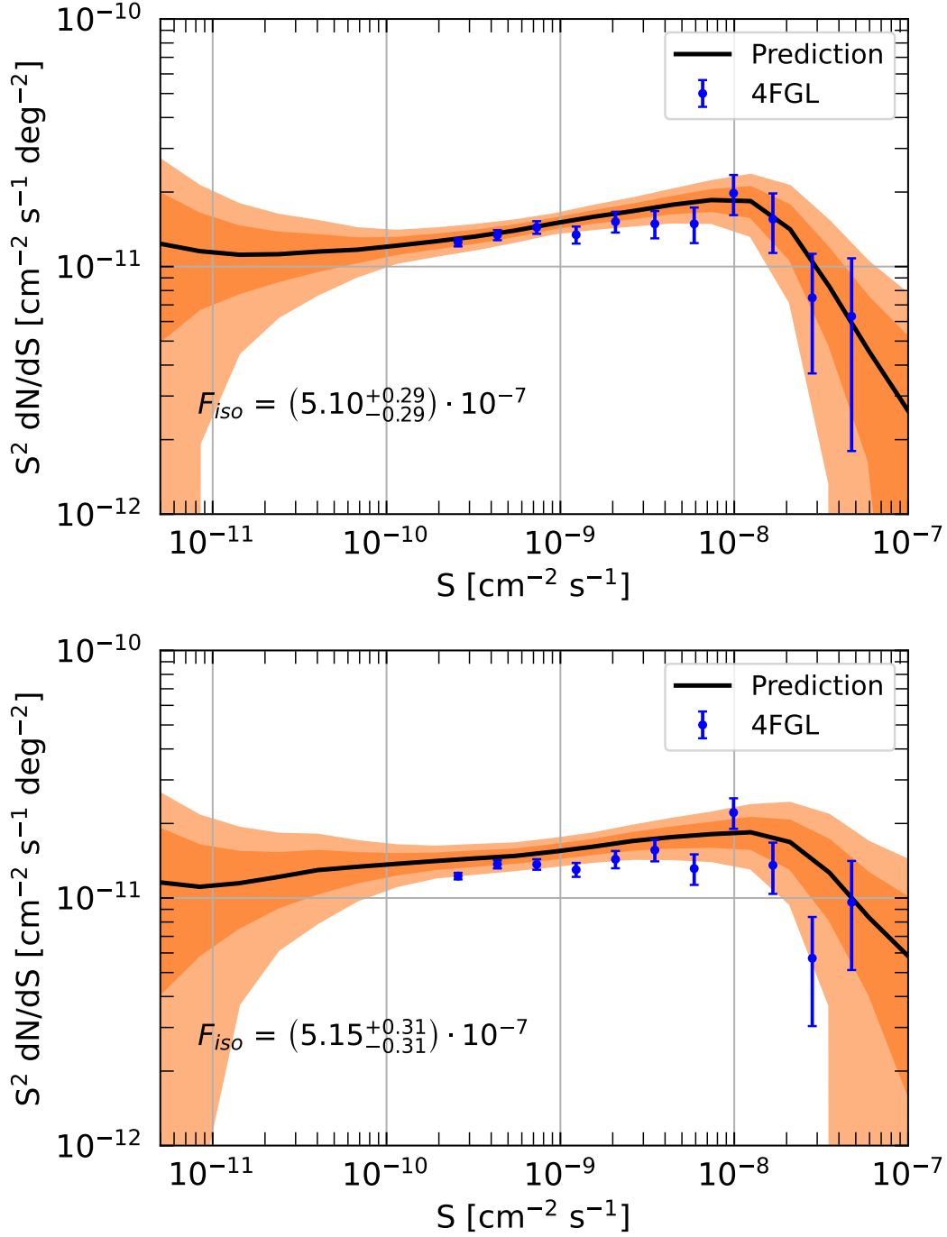
Fig. 6.18. Same as Figure 6.15 but for a latitude cut of 40° and 50°. The blue datapoints of the dN/dS of the 4FGL sources have been updated using only the source in the given region of interest.
