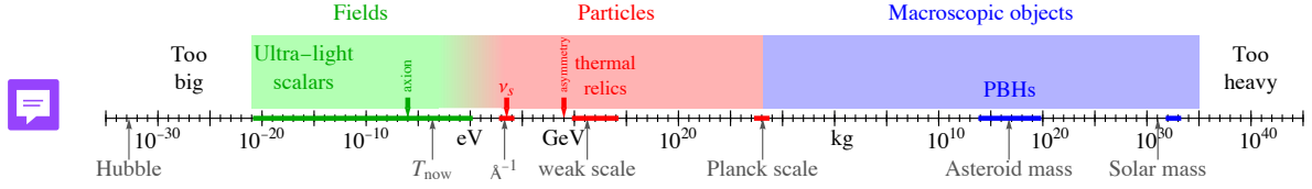
Fig. 1.5. The dark-matter mass landscape: viable candidate masses span roughly ninety orders of magnitude, from ultra-light bosonic fields to macroscopic primordial black holes. Each class is characterized by a distinct production mechanism and probed by a complementary set of experiments. Credit: Cirelli et al. [11]. [AA: consider replacing with a custom figure for the final version]
