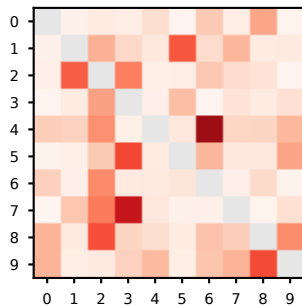
Decision Tree
