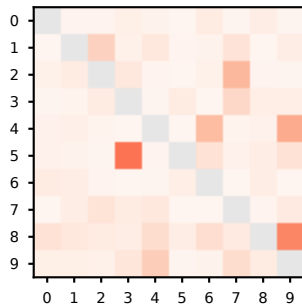
Logistic Regression
