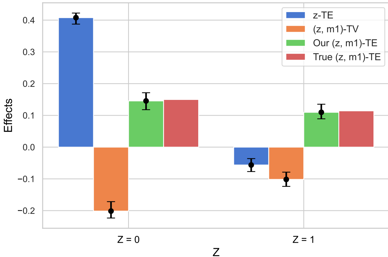
Effects Conditioned on Z
