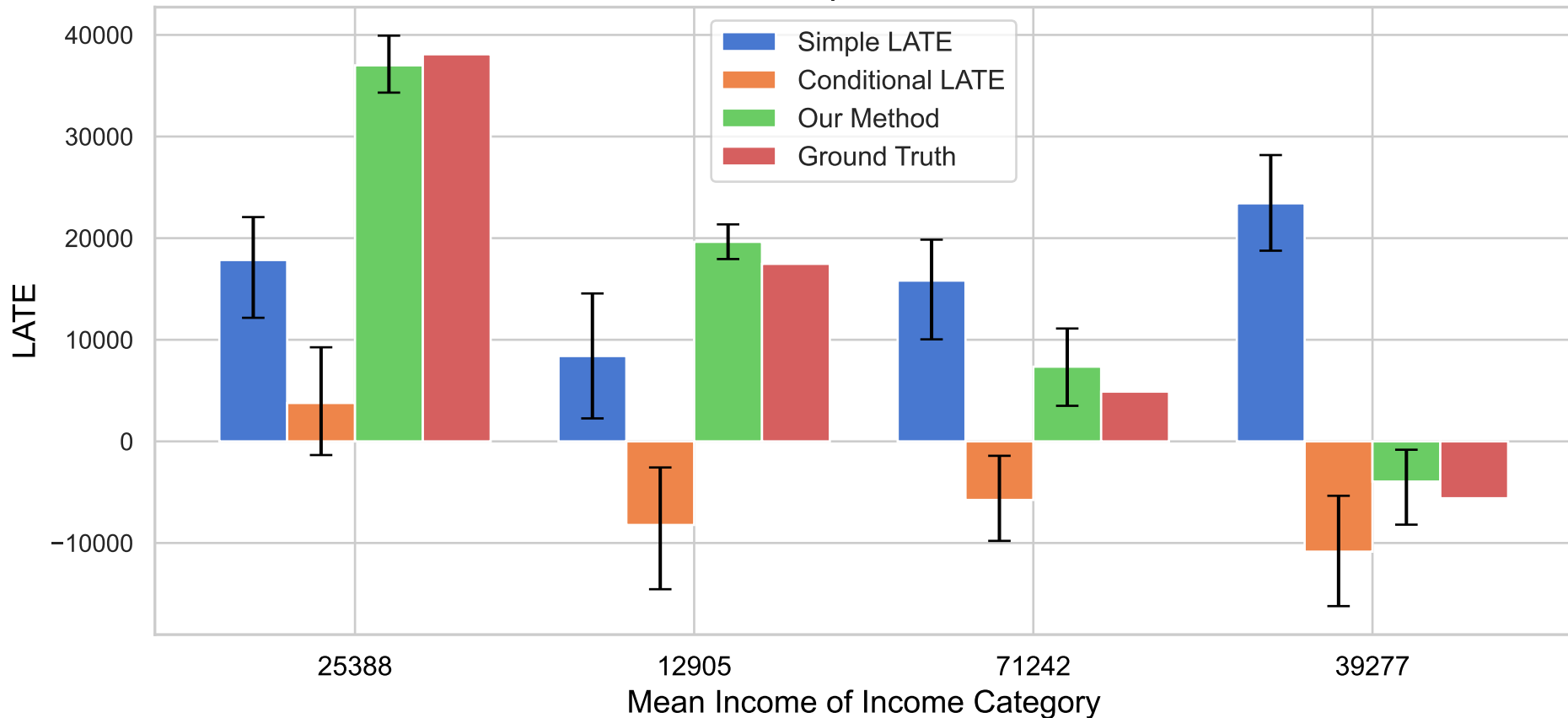
Income Specific Effects
