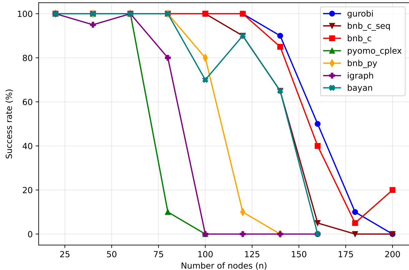
LFR Success Rate vs Graph Size (timeout=30s)
