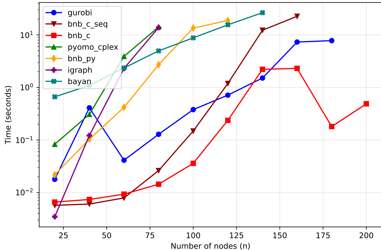
LFR Scaling: Median Time vs Graph Size
