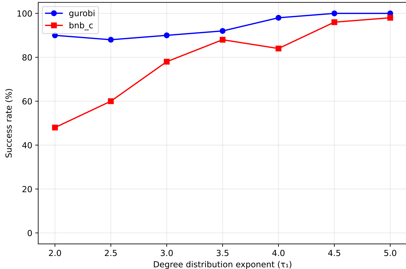
LFR Success Rate vs Degree Distribution Exponent (timeout=30s)
