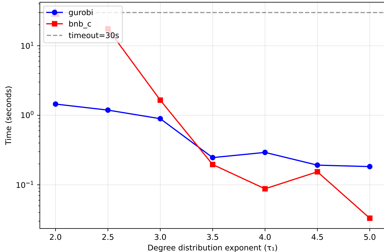
LFR: Median Time vs Degree Distribution Exponent
