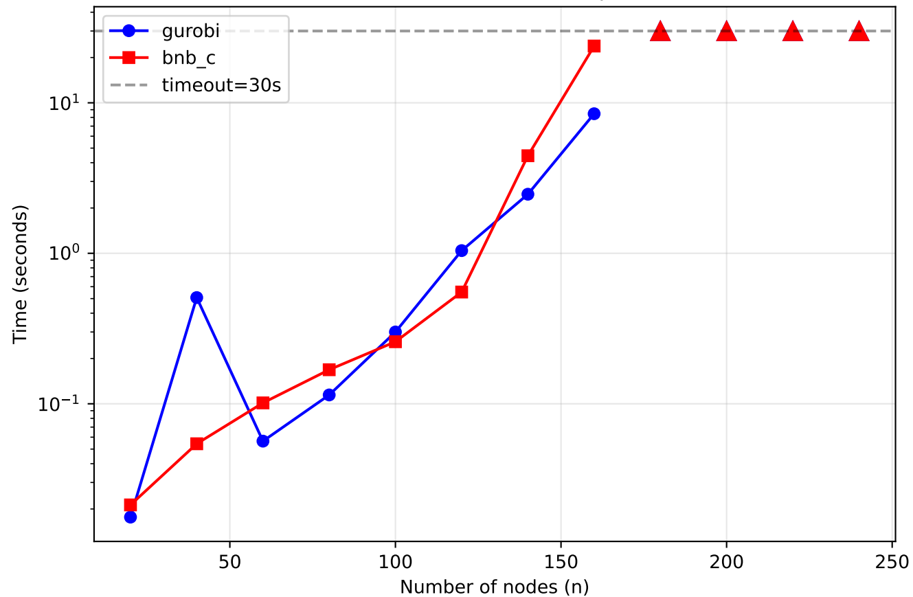
ABCD Median Time vs Graph Size
