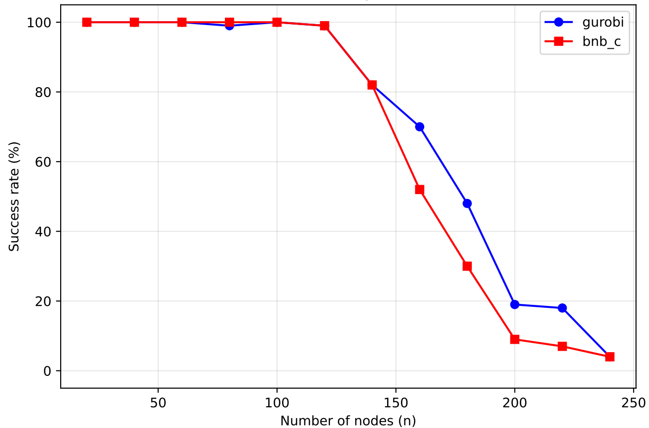
ACBD Success Rate vs Graph Size (timeout=30s)
