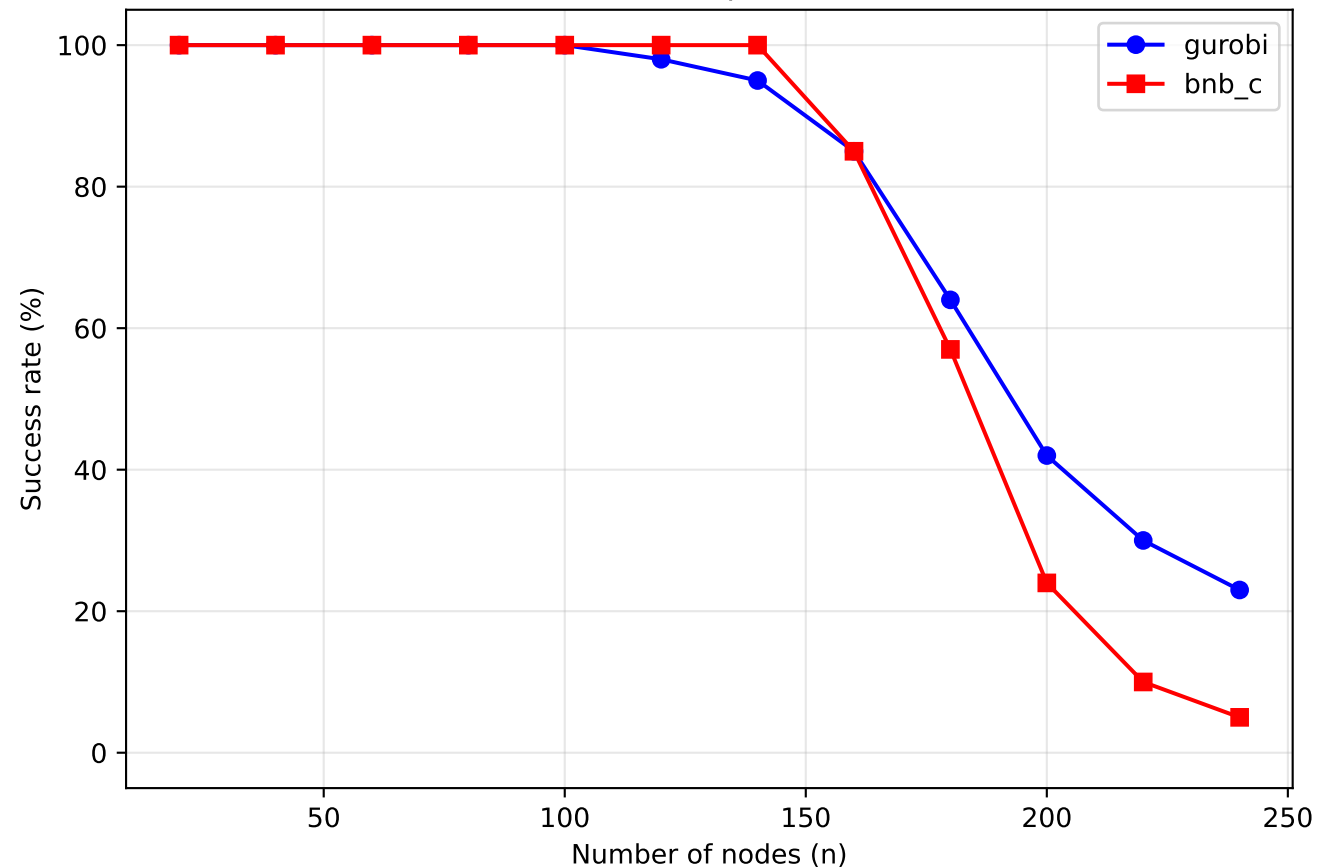
LFR Success Rate vs Graph Size (timeout=30s)
