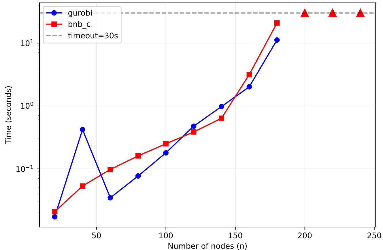
LFR Median Time vs Graph Size
