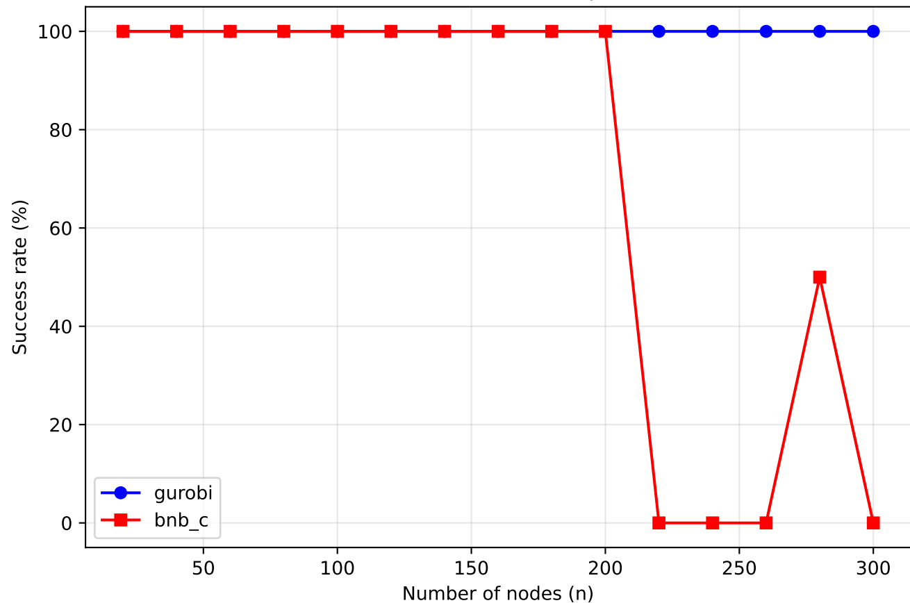
Planted Partition Success Rate vs Graph Size (timeout=5s)
