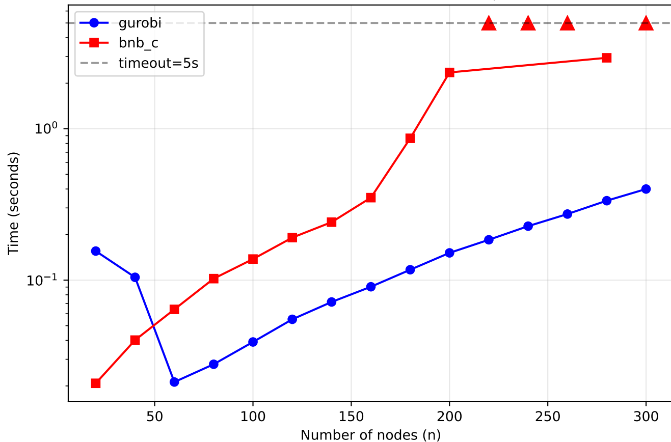
Planted Partition Median Time vs Graph Size
