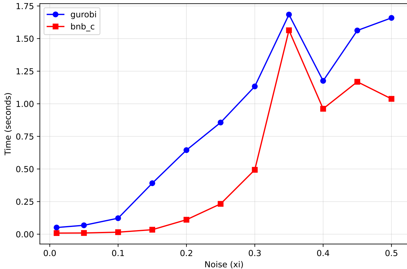
ABCD Median Time vs Noise Between clusters
