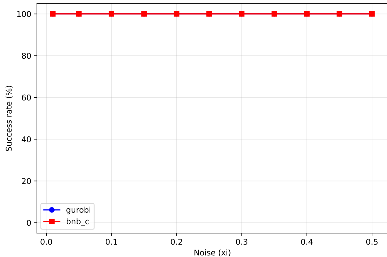
ACBD Success Rate vs Noise Between clusters (timeout=43s)
