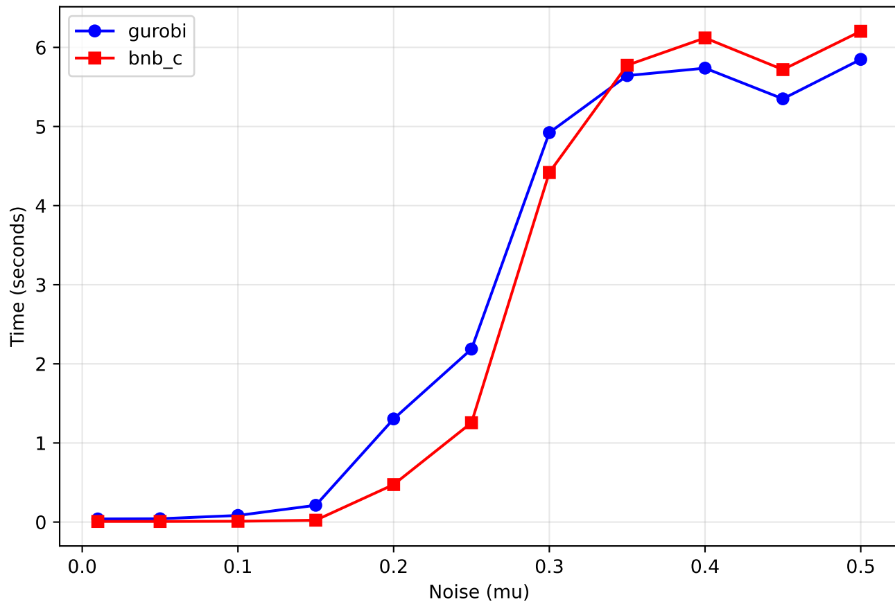
LFR Median Time vs Noise Between Clusters
