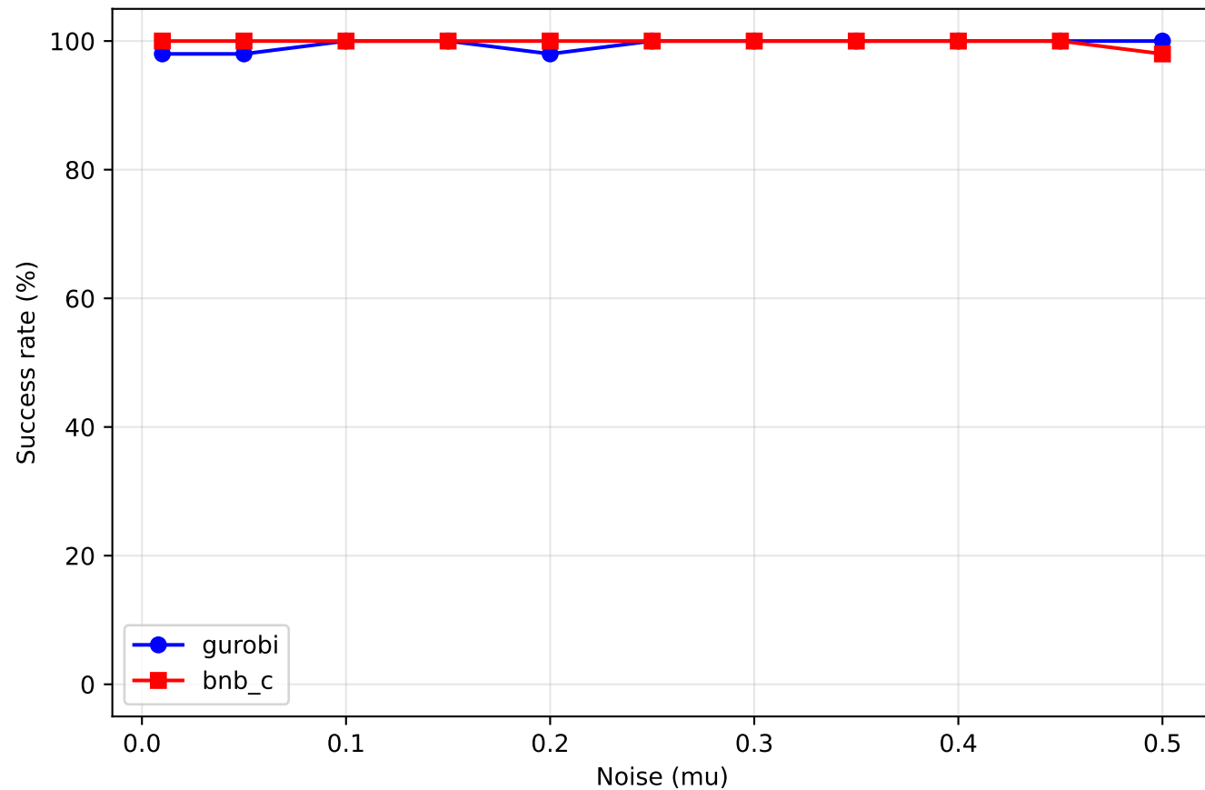
LFR Success Rate vs Noise Between Clusters (timeout=120s)
