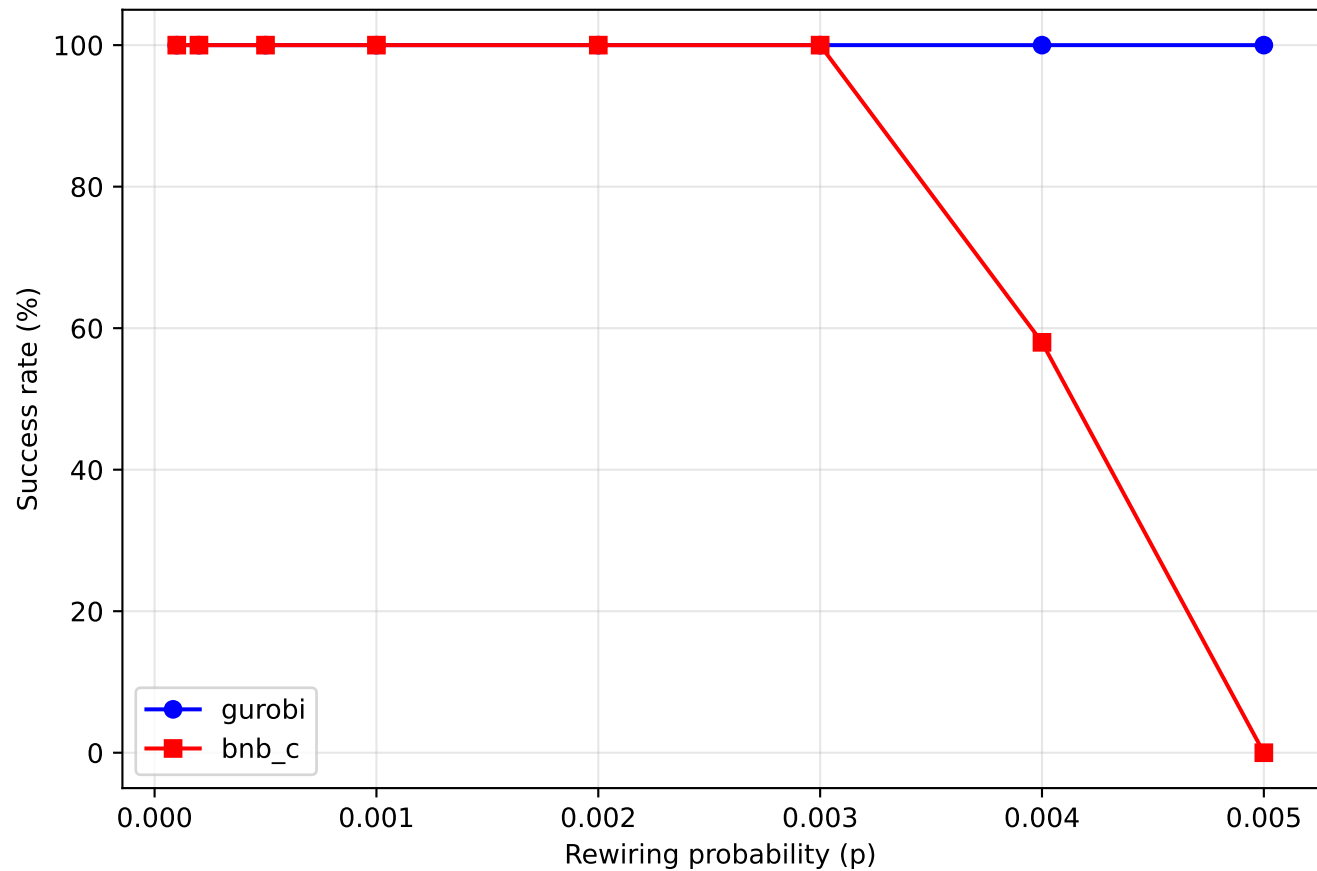
Relaxed Caveman Success Rate vs Noise (timeout=30s)
