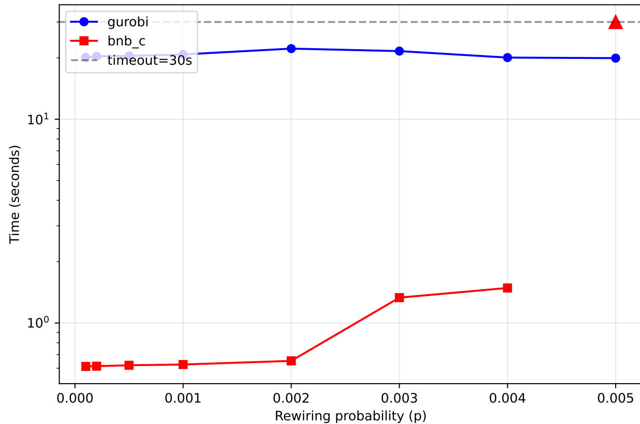
Relaxed Caveman Median Time vs Noise
