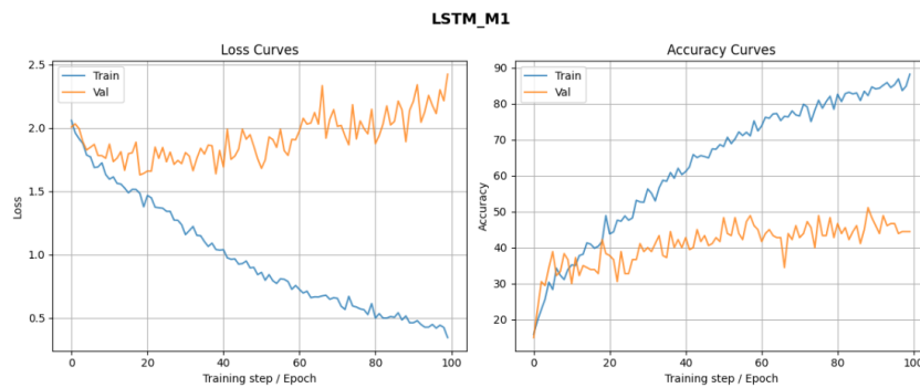
Figure 15: LSTM_M1: Loss and accuracy curves, 100 epochs.
