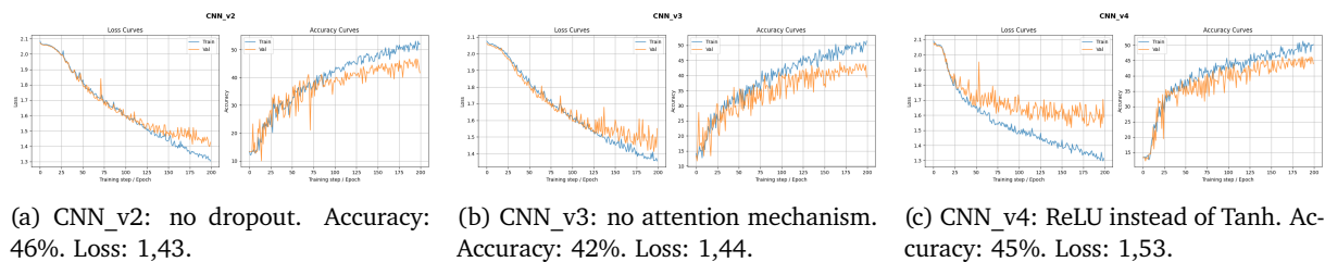
Figure 10: Loss and accuracy curves of each training performed for the ablation study.
