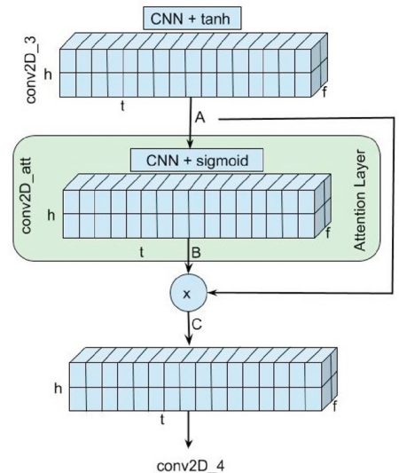
Figure 7: Attention mechanism component from Wijayasingha and Stankovic 2021. With B = \sigma(\text{conv2D}_{att}(A)) and C = A * B .
