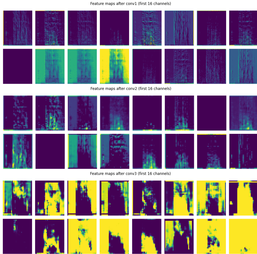
Figure 13: Feature maps for a specific input on the first three convolutional layers.
