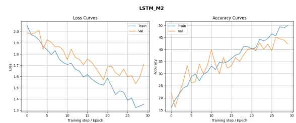
(b) LSTM_M2: Loss and accuracy curves
