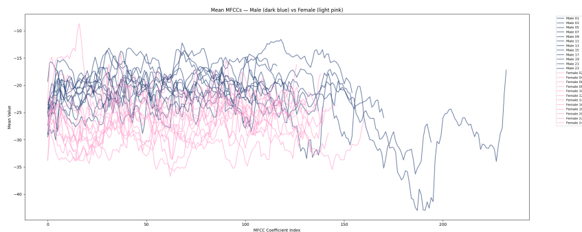
Figure 5: Mean MFCC features of all speakers in the train set saying the same sentence in the same emotion. Female speakers in pink; male speakers in navy.
