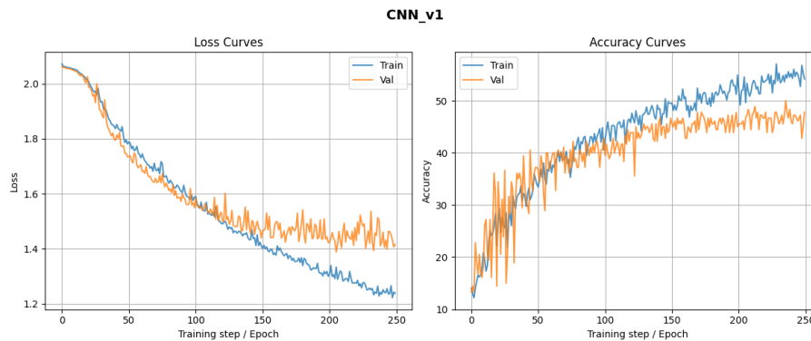
Figure 9: CNN training curves obtained from the Original Architecture in Wijayasingha and Stankovic 2021 with no changes. Peak accuracy: 51.1%
