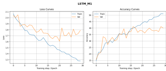
(a) LSTM_M1: Loss and accuracy curves
