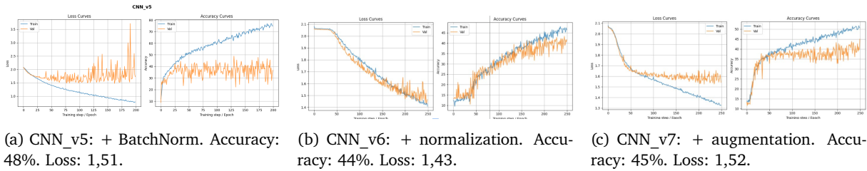
Figure 11: Loss and accuracy curves of each training performed by adding the respective components.
