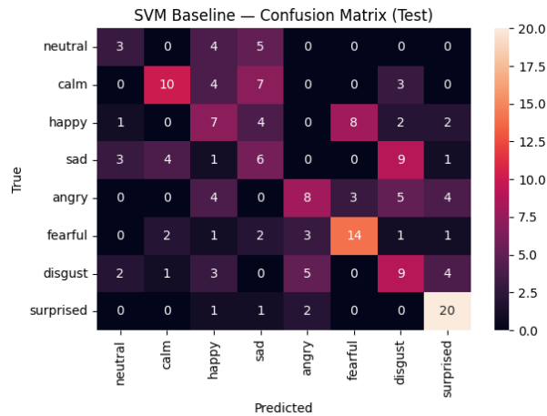
Figure 8: SVM Baseline Confusion Matrix on the test set.
