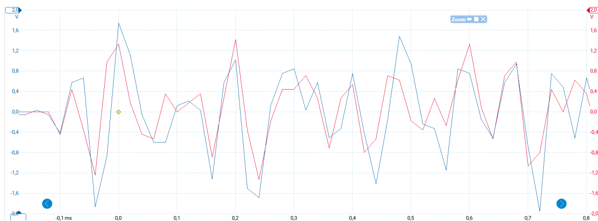
Figure 16: Onde transversale
