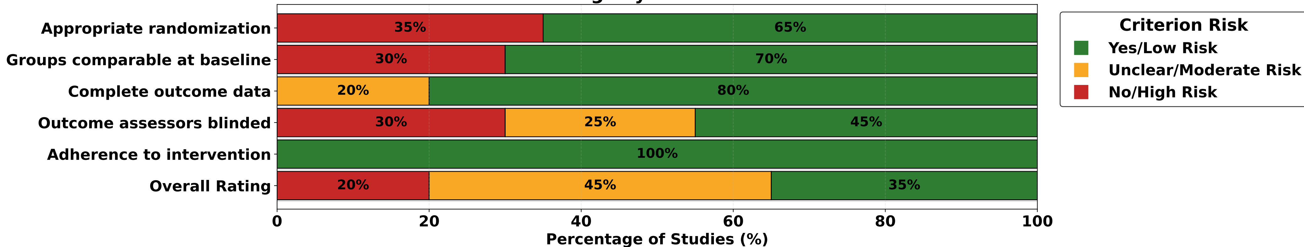
Distribution of Ratings by Criterion - Non-randomized
