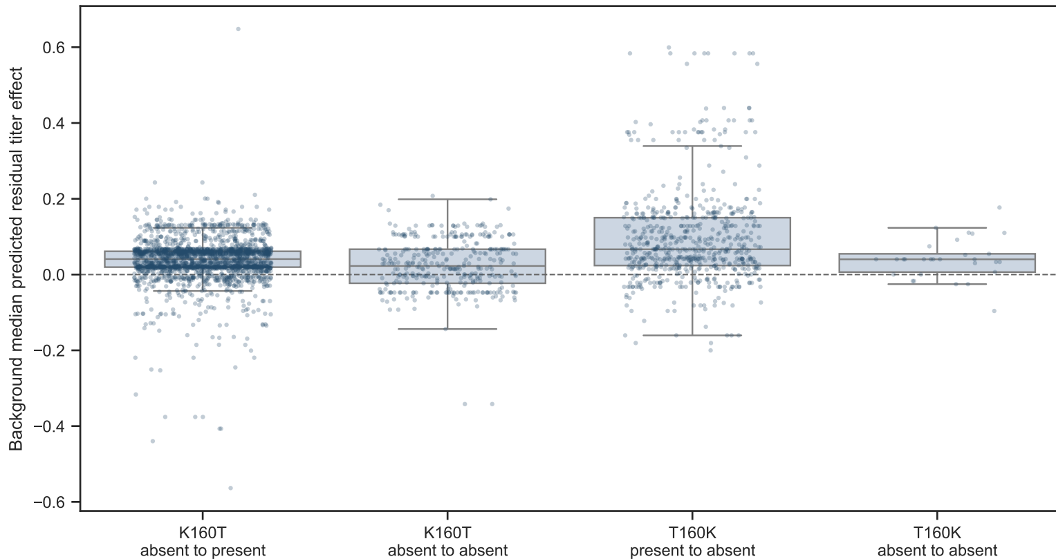
WIC filtered site-state model: HA1 158-160 glycosylation context
