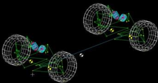
Suspension geometry-Lotus Shark
