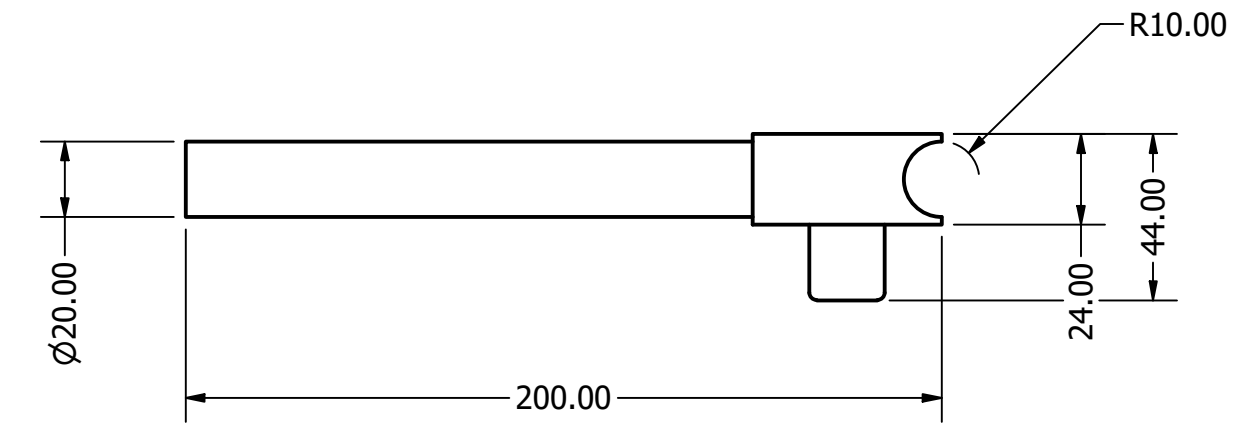
Lever SCALE 1 / 2
