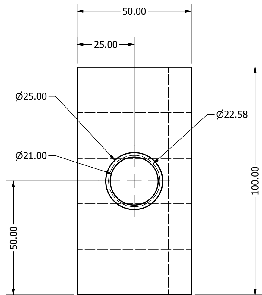
Base SCALE 1 / 2
