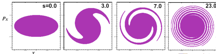
Figure 2: Root-mean-square (rms) emittance growth under nonlinear forces.
