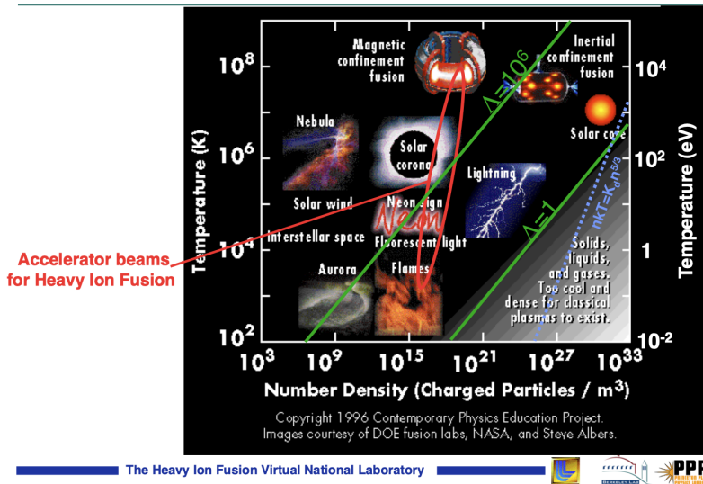
Figure 1: Plasmas characterized by temperature and number density. Green lines indicate constant plasma parameter \Lambda . [Updated version?]
