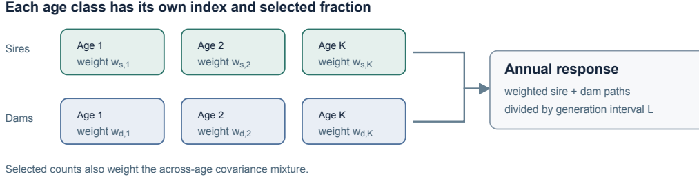
Figure 7: Selected age classes determine each parental path, the generation interval, and the covariance mixture. Editable SVG source: selection_ages.svg .
