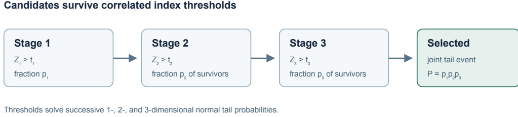
Figure 5: Conditional survival across stages; the final selected set is the intersection of all stage-tail events. Editable SVG source: selection_stages.svg .
