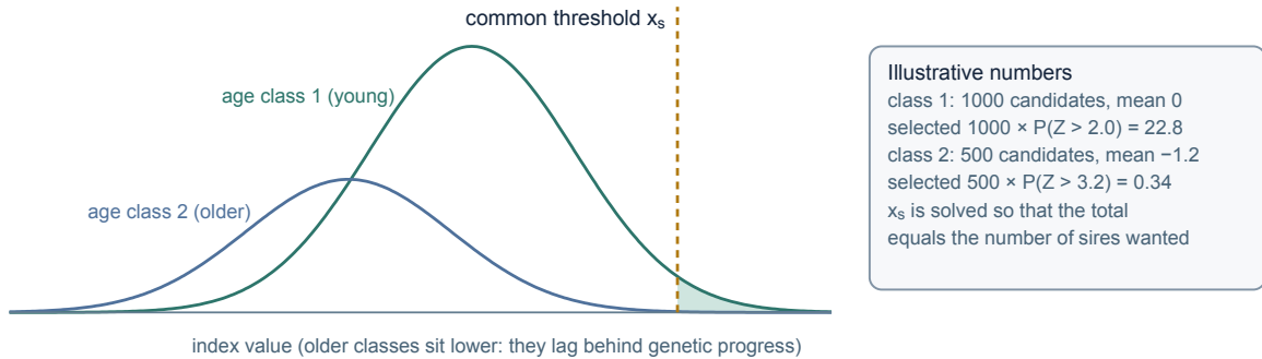
Figure 6: One threshold applied to two age classes of sires (illustrative numbers). The older class lags behind and contributes few selected animals even though it is large. Editable SVG source: selection_agerthreshold.svg .
