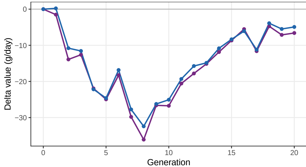
D Phenotype vs Total GV -- social drag
