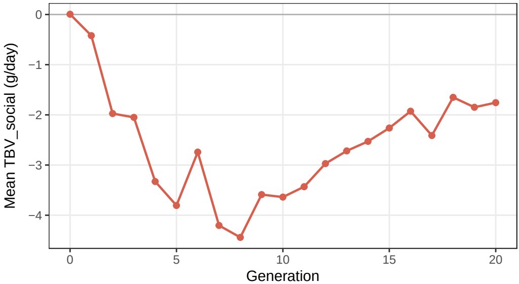
C Mean TBV_social (raw) -- correlated response
