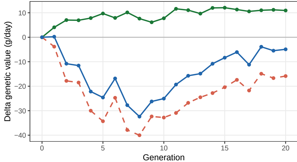
B Genetic trends (zero-centred at gen 0)
