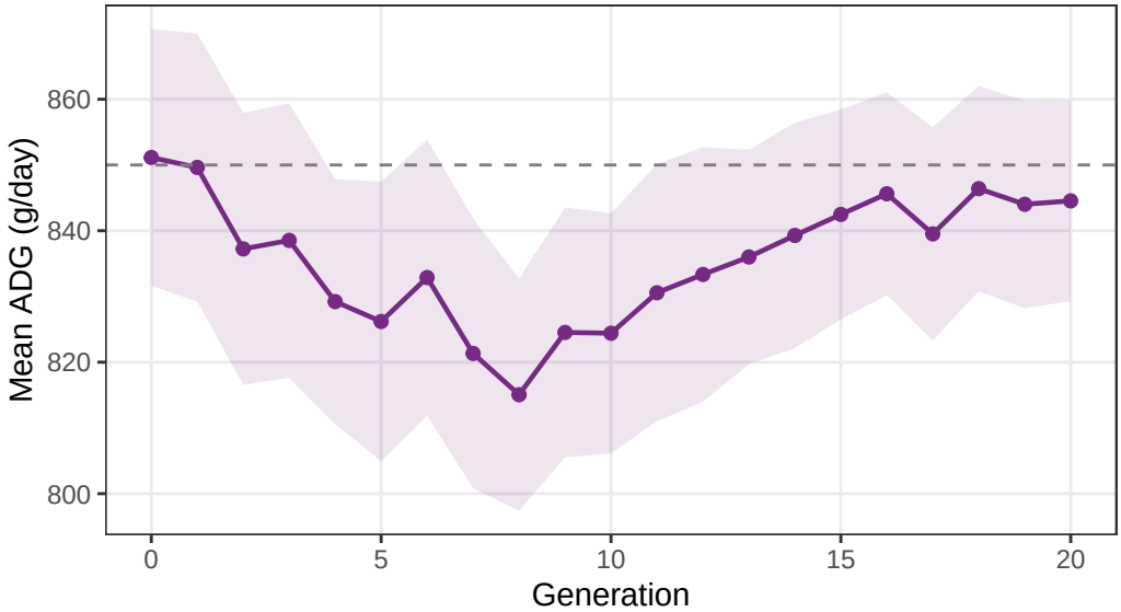
A Phenotypic mean ± 1 SD
