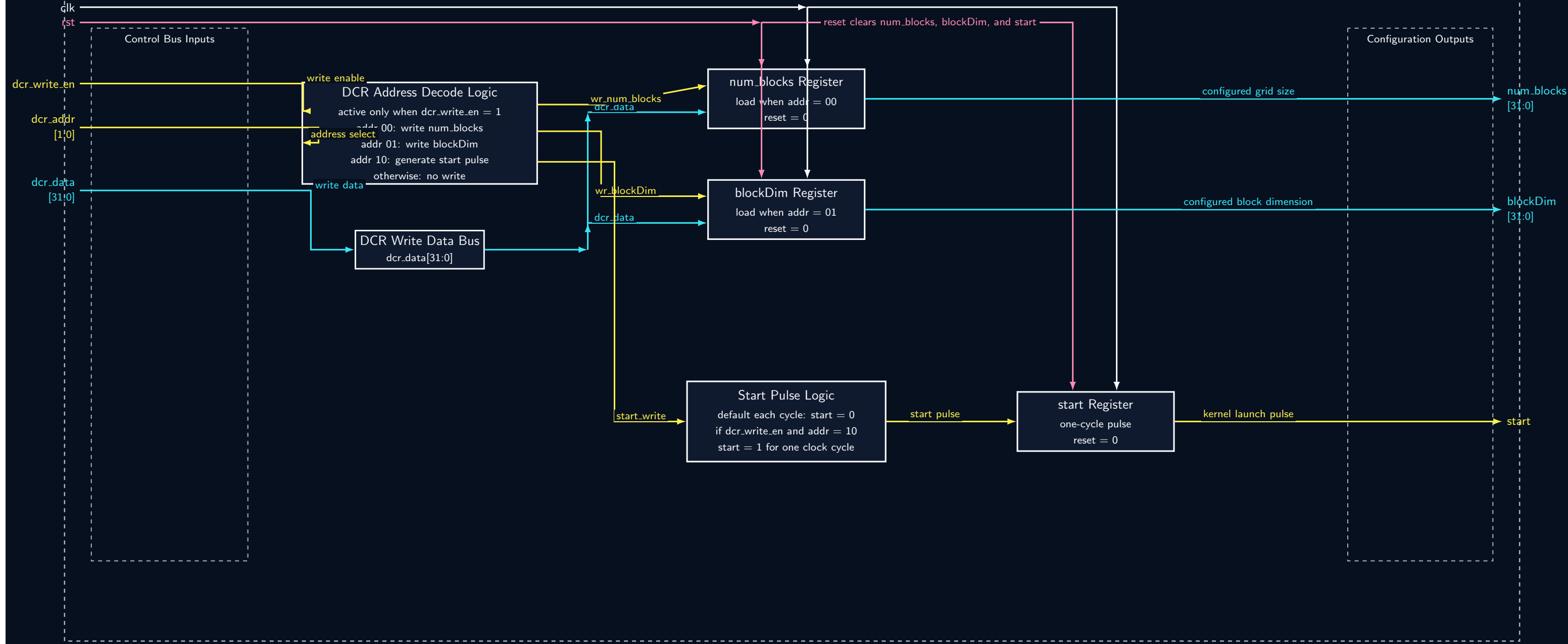
Device Control Register write decoder with configuration registers and start pulse generation
