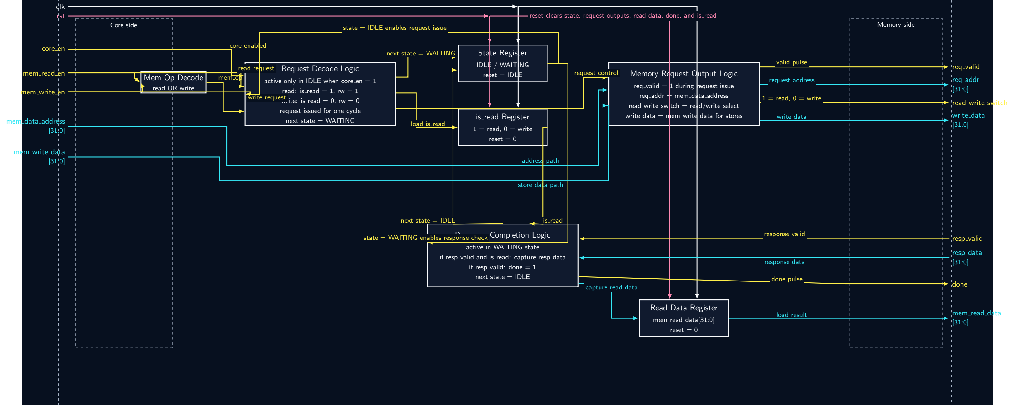
Load/Store Unit control path with request generation and response completion
