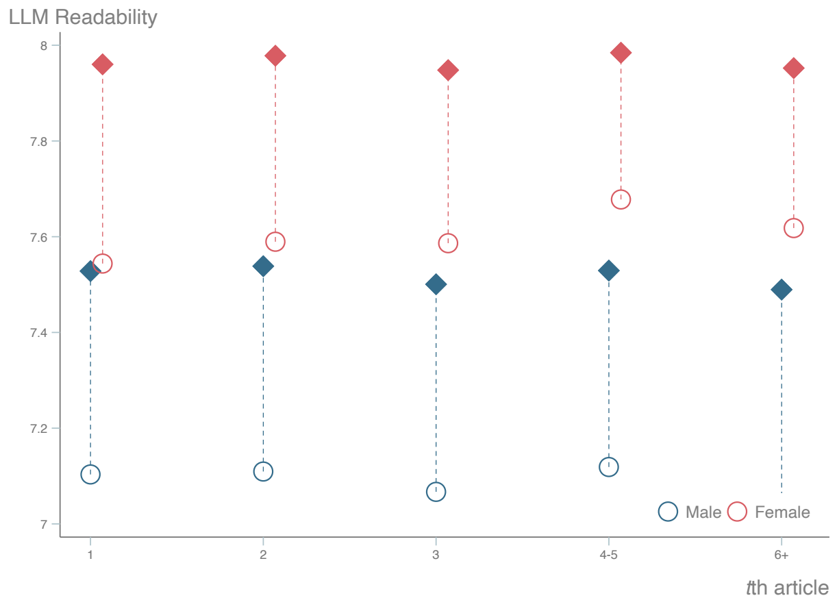
Figure 6: Figure 6 LLM
