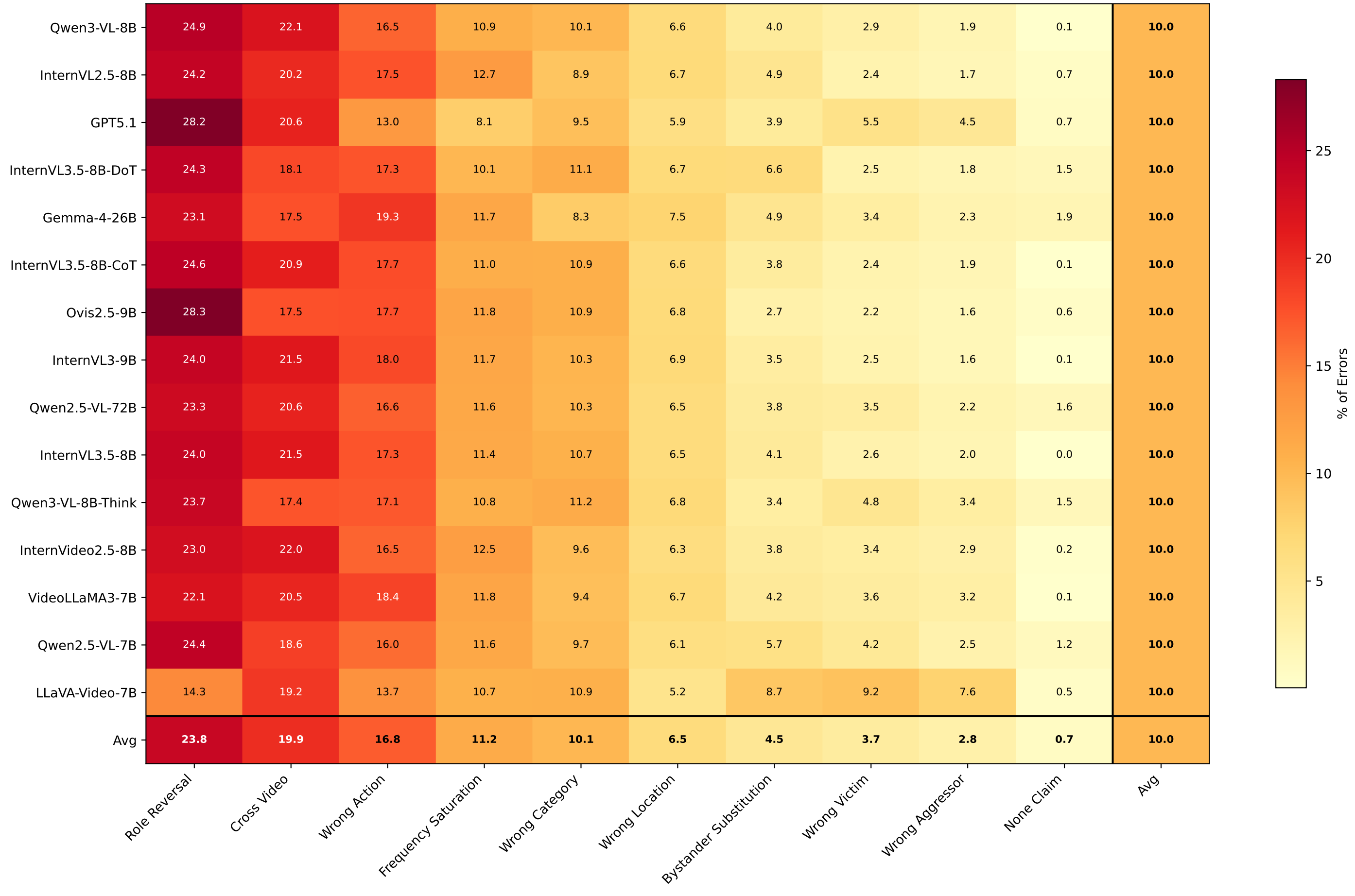
Distractor Vulnerability Heatmap (% of Errors)
