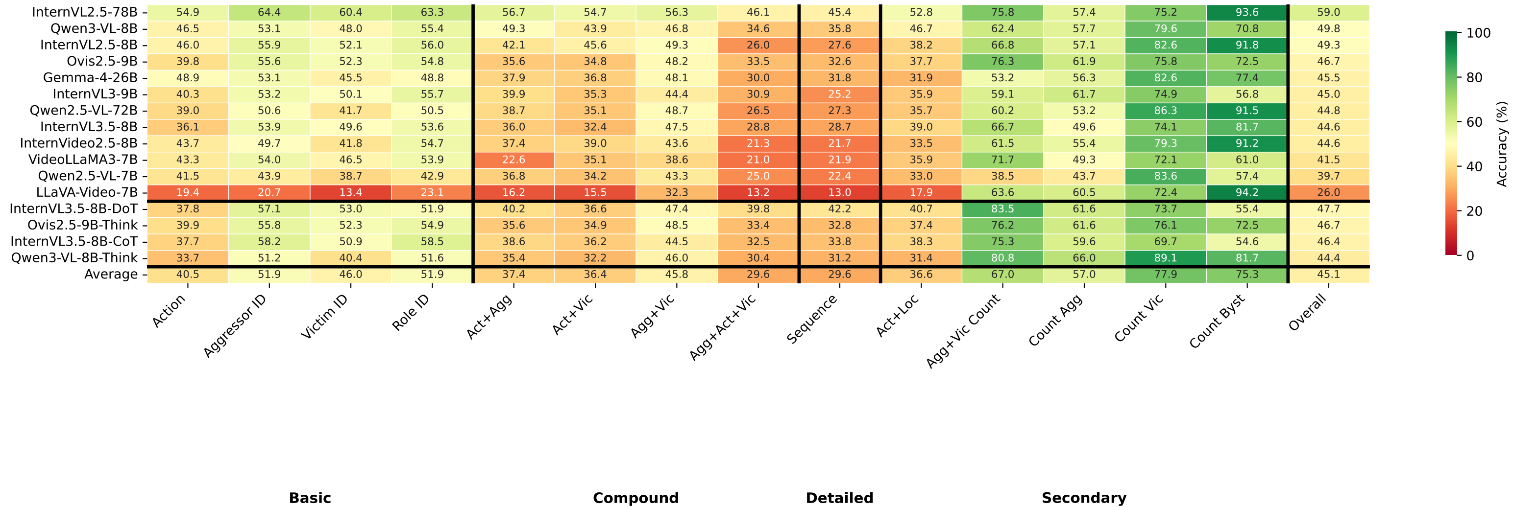
Model Accuracy by Question Type
