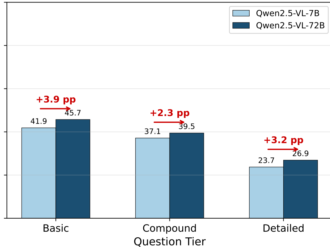
Qwen2.5-VL
