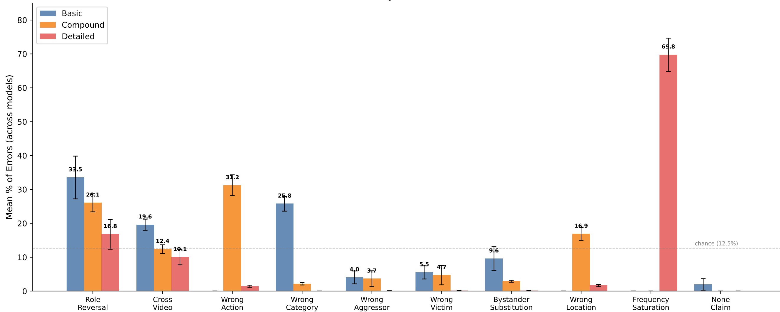
Distractor Vulnerability Shift Across Question Tiers
