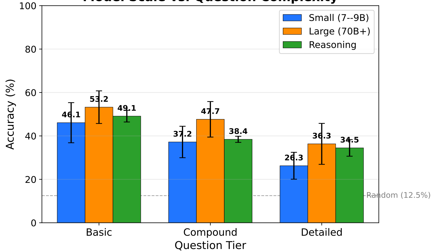
Model Scale vs. Question Complexity
