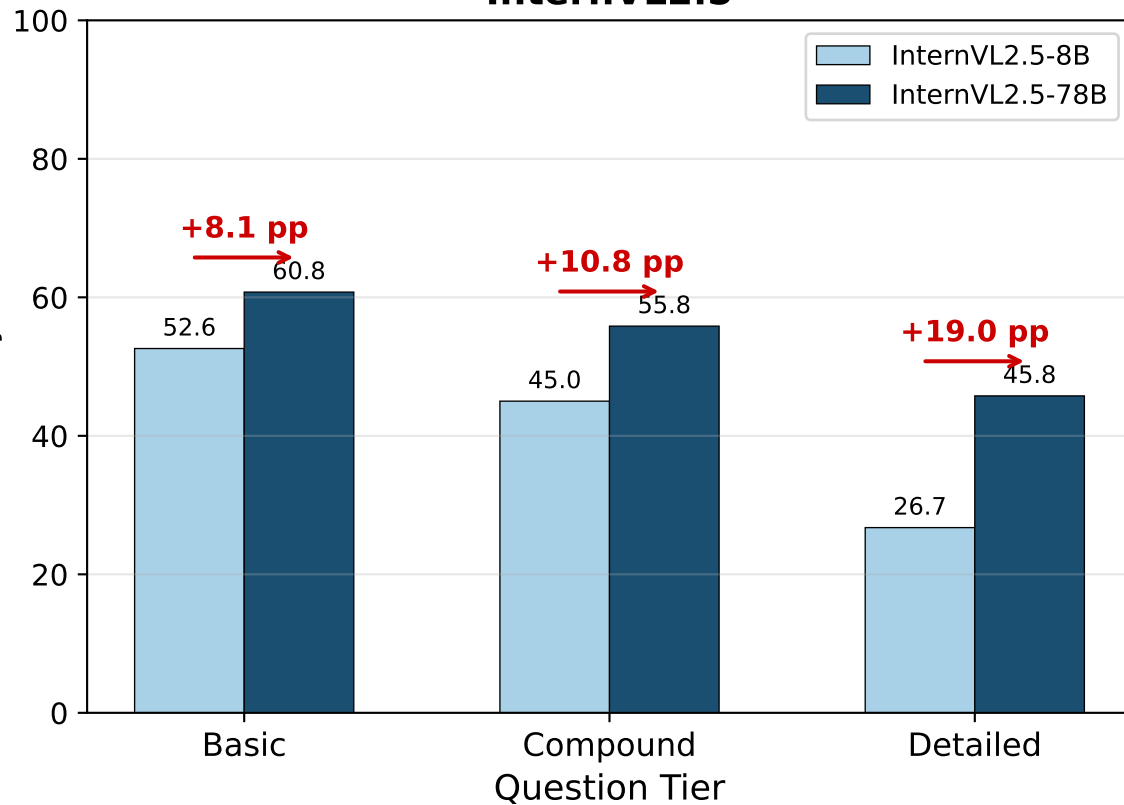
InternVL2.5
