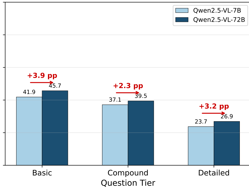
Qwen2.5-VL
