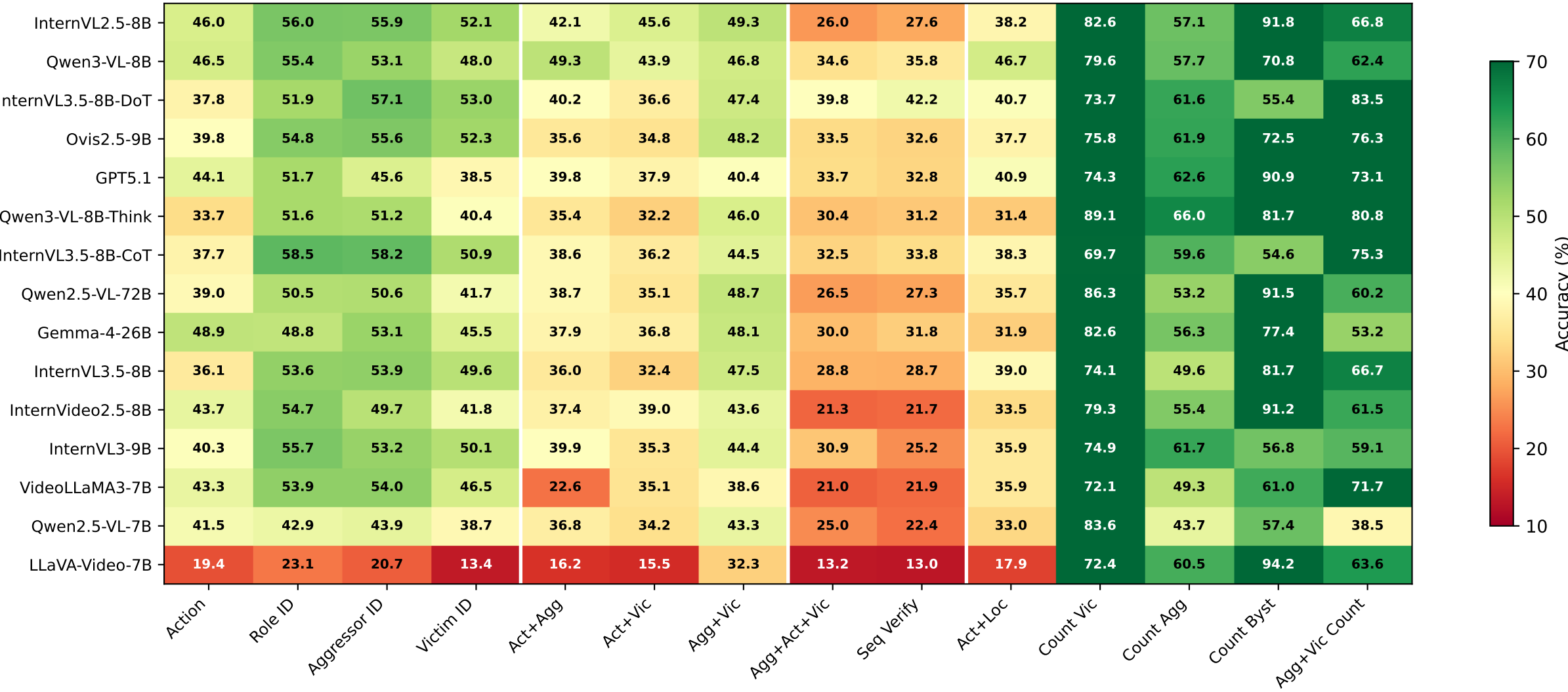
Basic Compound Detailed Secondary Model Accuracy by Question Category (%)
