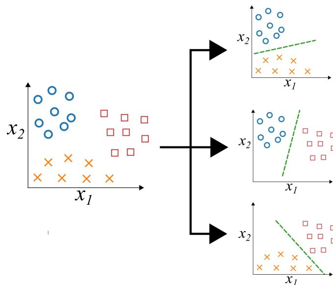
Figure 4.14: One-versus-one (OvO) classifier for a multi-class dataset.
