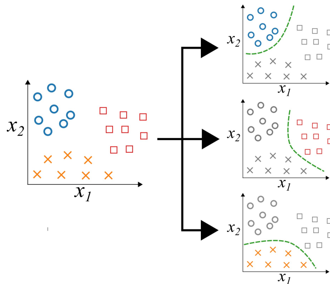
Figure 4.13: One-versus-Rest (OvR) classifier for a multi-class dataset.
