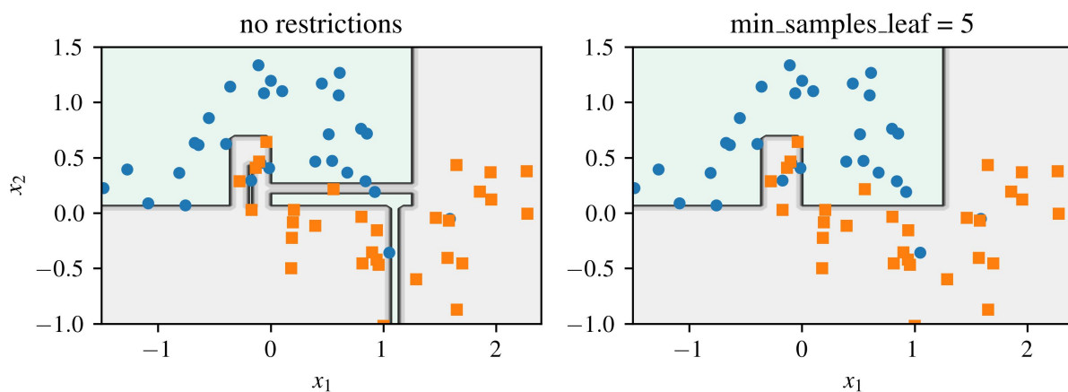
Figure 7.5: Regularization effects using min_samples_leaf
