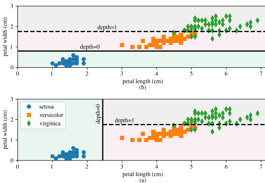
Figure 7.10: Decision Tree Sensitivity to initial conditions, showing: (a) random number generator seeded with “1”, and: (b) random number generator seeded with “2”. a
