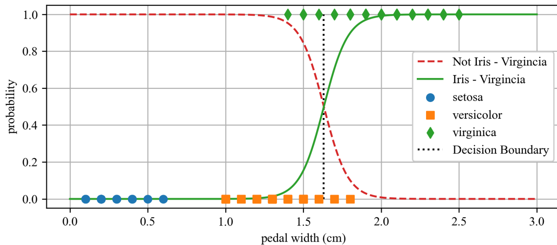
Figure 5.5: Decision boundary for the flowers of three Iris plant species with C set to C = 10^{10} .
